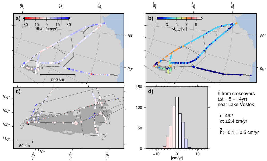
Figure 2. a) Elevation change rate \dot{h} from crossovers between different seasons (20 km block mean values). b) Maximum observation time span of crossover differences within each block. c) \dot{h} in the Lake Vostok region. Crossovers on the convoy track or with \Delta t < 5 yr are considered uncertain and thus plotted half sized. d) Distribution of the valid crossovers ( \Delta t \geq 5 yr, no anthropogenic surface disturbances) in the Lake Vostok region (100–108.5 °E, 76–79 °S).
