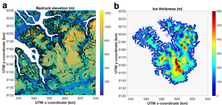
10 Figure 2. (a) Bedrock elevation (Starzer and Reeh, 2001). Areas below sea level (fjords with semi permanent sea-ice) are depicted in white, the thick black line corresponds to the outline of the observed glaciated area. (b) Ice thickness in the mid 1990s based on the DEM from Starzer and Reeh (2001).
