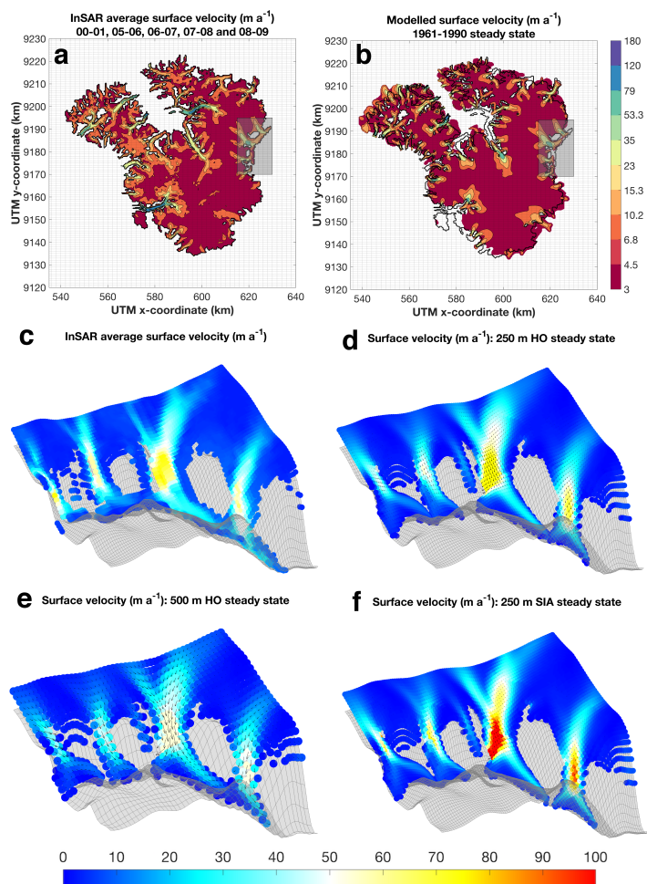
Figure 7. (a) InSAR derived surface velocities (Joughin et al., 2010, 2015) and (b) 1961-1990 steady state surface velocities (250-m HO run). Black lines represent the observed ice cap outline from the Starzer and Reeh (2001) DEM, the shaded box delineates the area shown in (c,d,e,f). (c) InSAR derived surface velocities, (d) 250 m HO surface velocities, (e) 500 m HO surface velocities and (f) 250 m SIA surface velocities. For the InSAR velocities (c) the geometry corresponds to the observed one (Starzer and Reeh, 2001), while for the model runs (d,e,f) the geometry corresponds to the steady state geometry.
