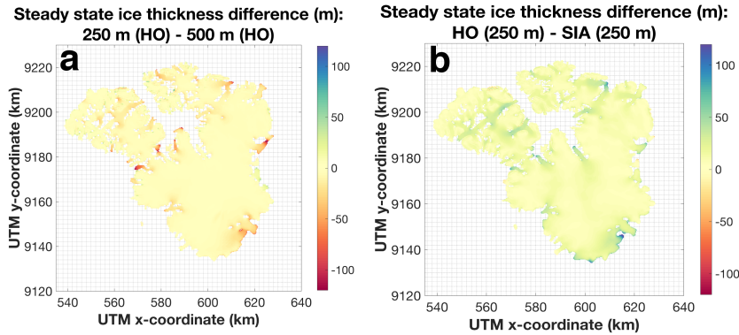
Figure 8. (a) Difference in ice thickness between 250 m and 500 m HO steady states and (b) difference in ice thickness between HO and SIA steady states (at 250 m).
