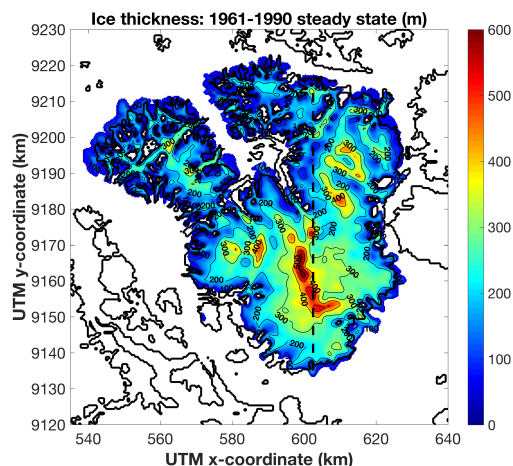
Figure 5. 1961-1990 steady state ice thickness from the HO 250-m resolution run. The thick black lines represent the outlines from the glaciated areas from the DEM (Starzer and Reeh, 2001). The dotted black line is the transect at X UTM = 602.5 km that is illustrated in Figure 11 .
