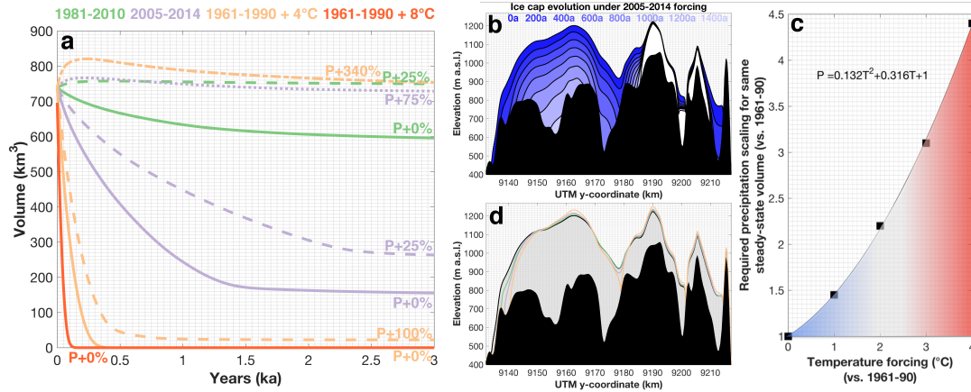
Figure 11. (a) Volume evolution of Hans Tausen Iskappe under different climatic conditions. The solid lines represent simulations where the precipitation is unaltered (i.e. P+0%), while the dotted lines represent simulation with a modified precipitation. The starting point of all simulations is the 1961-1990 steady state geometry. (b) Evolution of the Hans Tausen Iskappe along UTM x= 602.5 km transect under the 2005-2014 forcing, starting from the 1961-1990 steady state, for 200 year time intervals. The black area represents the bedrock and the white area represent the final steady state geometry. The location of the transect is shown in Figure 5 . (c) Temperature forcing and corresponding precipitation forcing (scale factor) needed for 1961-1990 steady state volume to be preserved. The polynomial fit is based on 5 simulations (1961-1990 +0/1/2/3/4°C), which are represented by the black dots. The blue area broadly corresponds to the range where an attenuation of the mass loss is possible, whilst the red area represent the range under which the ice cap is to (largely) disappear. (d) Ice cap profiles along the UTM x = 602.5 km transect. The shaded grey area is the 1961-1990 steady state ice cap geometry. The 3 other geometries correspond to the 1981-2010 (P+25%), 2005-2014 (P+75%) and 1961-1990 +4°C (P+340%) steady states and follow the same colour scheme as in (a). The location of the transect is shown in Figure 5 .
