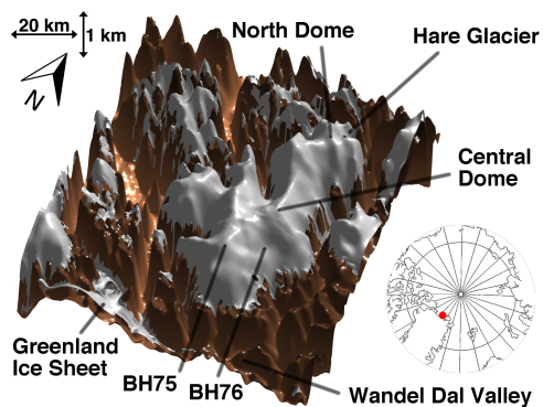
Figure 1. Hans Tausen Iskappe in the mid 90s. Figure created with the TopoZeko toolbox (Zekollari, 2016). Map in lower right corner shows the location (red dot) of the ice cap in Greenland.
