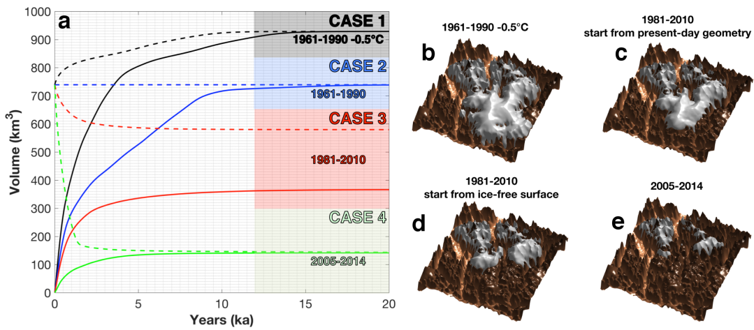
Figure 9. (a) Volume build-up of Hans Tausen Iskappe for different initial states (ice free surface and 1961-1990 steady state geometry) and under different climatic conditions. The four coloured regions (cases) represent clusters of simulations with a similar build-up and thresholds in the system and are defined and discussed in the text. (b,c,d,e) Modelled steady state geometry for different climatic forcings (figures made with TopoZeko toolbox (Zekollari, 2016))
