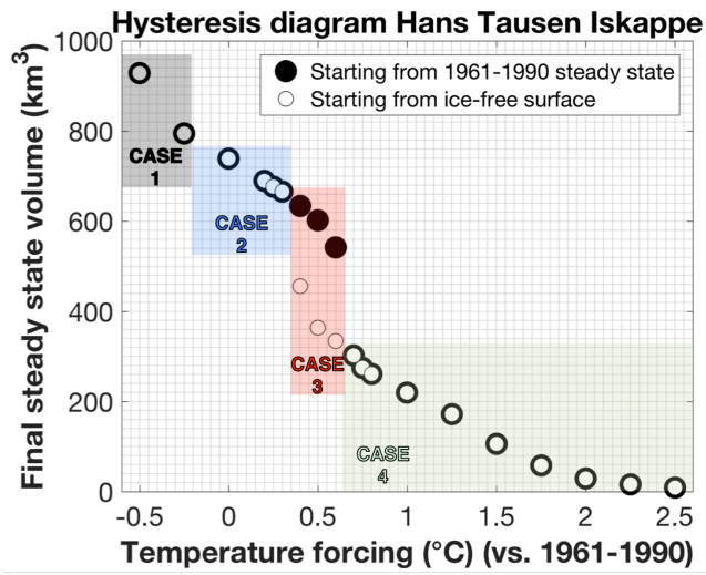
5 Figure 10. Final steady state volumes under different climatic conditions and for different starting geometries. The four cases are the same as in Figure 9 and are described in the text. Bold circle outlines mean that the final steady state is independent from the initial conditions.
