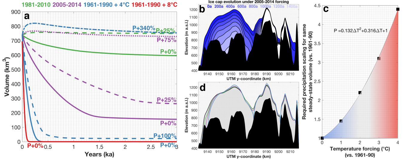
Figure 11. (a) Volume evolution of Hans Tausen Iskappe under different climatic conditions. The solid lines represent simulations where the precipitation is unaltered (i.e. P+0%), while the dotted lines represent simulation with a modified precipitation. The starting point of all simulations is the 1961-1990 steady state geometry. (b) Evolution of the Hans Tausen Iskappe along UTM x= 602.5 km transect under the 2005-2014 forcing, starting from the 1961-1990 steady state, for 200 year time intervals. The black area represents the bedrock and the white area represent the final steady state geometry. The location of the transect is shown in Figure 5 . (c) Temperature forcing and corresponding precipitation forcing (scale factor) needed for 1961-1990 steady state volume to be preserved. The polynomial fit is based on 5 simulations (1961-1990 +0/1/2/3/4°C), which are represented by the black dots. The blue area broadly corresponds to the range where an attenuation of the mass loss is possible, whilst the red area represents the range under which the ice cap is to (largely) disappear. (d) Ice cap profiles along the UTM x = 602.5 km transect. The shaded grey area is the 1961-1990 steady state ice cap geometry. The 3 other geometries correspond to the 1981-2010 (P+25%), 2005-2014 (P+75%) and 1961-1990 +4°C (P+340%) steady states and follow the same colour scheme as in (a). The location of the transect is shown in Figure 5 .
