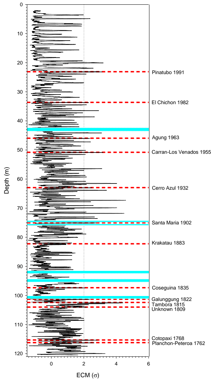
Fig. 5. Continuous record of ECM (except for six measurement gaps shown as cyan bands). Normalized conductivity (black line) is expressed as multiple of standard deviation ( \sigma ). The 2 \sigma threshold is shown as a dotted vertical line, and identified volcanic peaks as dashed red horizontal lines.
