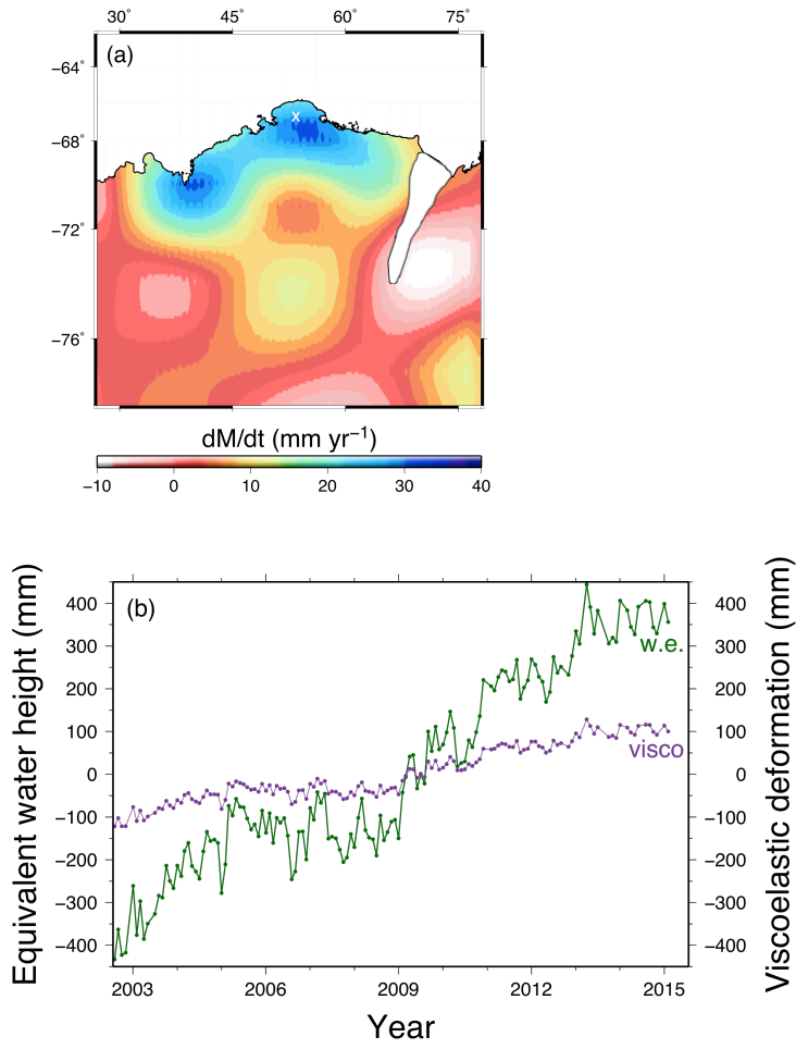
5 Figure 3: (a) Trend of the observed mass anomalies in Enderby Land monitored by GRACE over the time span of 2003-2009, uncorrected for GIA. The white cross illustrates the location of Richardson Lake, a former GPS station. (b) The time series shows a change in gravity at a chosen location in Enderby Land ( 67^\circ\text{S } 54^\circ\text{E} ) over the total observational period. The green line illustrates the change assuming the gravitational change is caused by a surface mass load and is expressed in water equivalent (w.e.) (Eq.1), the purple line illustrates a change due to viscoelastic deformation (GIA) (Eq.2).
