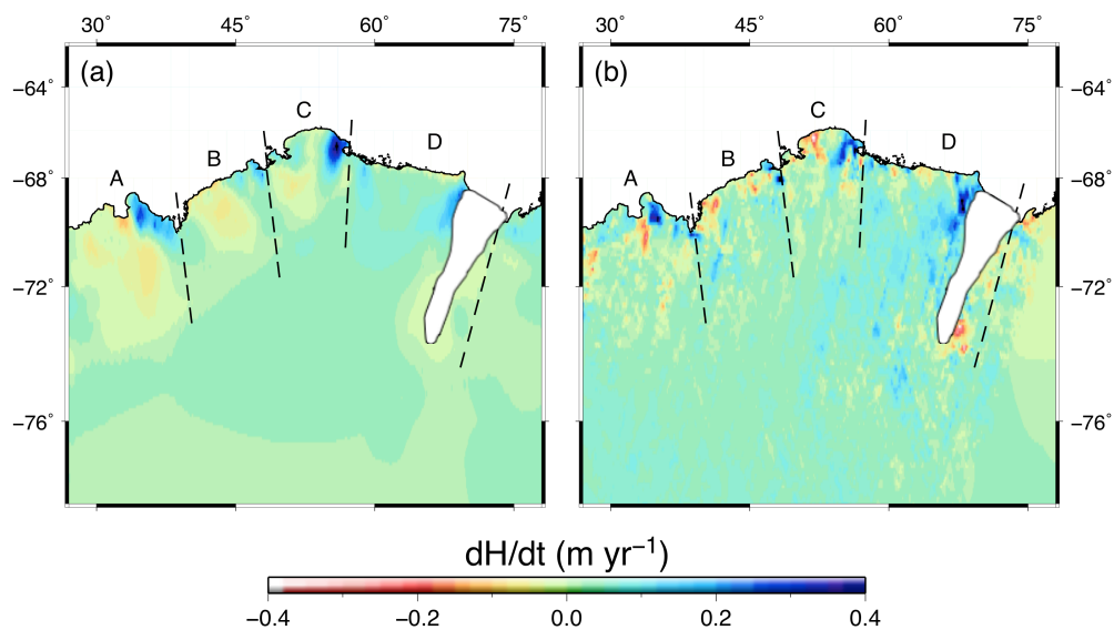
Figure 6: (a) our modelled rate of change of surface elevation retrieved by removing our estimated ice dynamic rates, obtained from GRACE, from the modelled trend in surface elevation (SMB-firn compaction) using RACMO2.3, compared to (b) the ICESat observations.
