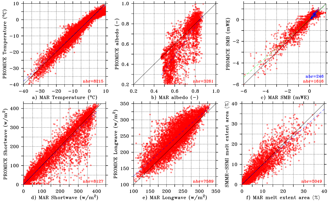
Figure 5. a) Scatter plot of the MAR ERA-Interim daily near-surface temperature versus near-surface daily temperature recorded by 12 AWS's from the PROMICE network over 2008-2010. The number of observations used here is listed in red and units are degrees Celsius. b) Same as a) but for the surface albedo. c) Scatter plot of the MAR ERA-Interim SMB (in mWE) with respect to ice core measurements in the accumulation area (in blue) and SMB measurements in the ablation (in red) from the PROMICE dataset over 1958-2010. We refer to the text for more details on how this comparison is performed. d) Same as a) for the shortwave downward radiative flux (in W/m 2 ). e) Same as d) for the longwave downward radiative flux. f) Daily melt extent (in % of the ice sheet area) simulated by MAR ERA-Interim over the 1979-2010 summers (May-September) versus the satellite derived one. More information about the thresholds used for retrieving the melt extent is given in the text.
