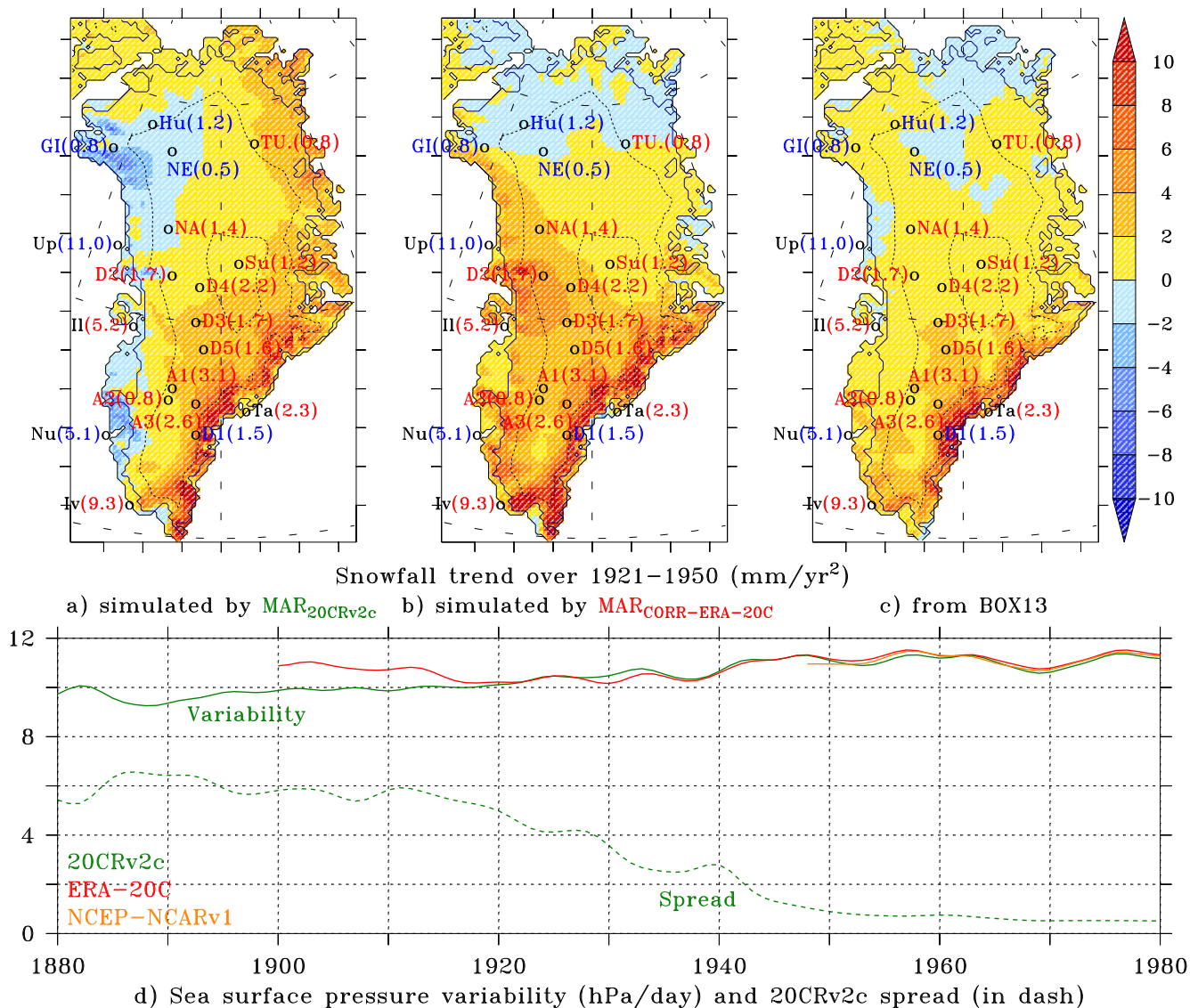
Figure 9. a) Annual snowfall trend (in \text{mmWE mm w.e./yr}^2 ) over 1921–1950 as simulated by MAR forced by 20CRv2c. The observed trend (in \text{mmWE mm w.e./yr}^2 ) from some locations listed in Mernild et al. (2015) are also pointed highlighted on the figure. These observed negative (resp. positive) trends are the values printed in blue (resp. in red) on the map. Trend of total precipitation (rain+snow) are also pointed in black for 5 coastal weather stations from DMI. b) Same as a) but for MAR CORR-ERA-20C . c) Same as a) but for BOX13. d) Time series of the annual mean daily variability (i.e. standard deviation of the daily values) of the sea level pressure around Greenland ( 0^\circ \text{ W} \leq \text{longitude} \leq 80^\circ \text{ W} and 55^\circ \text{ N} \leq \text{latitude} \leq 85^\circ \text{ N} ) from 20CRv2c (in green), ERA-20C (in red) and NCEPv1 (in orange). The ensemble mean spread (i.e. the standard deviation of the ensemble deviations at each time) from 20CRv2c over the same area is also plotted in dash. Finally, only 10yr-running means are shown for more readability.
