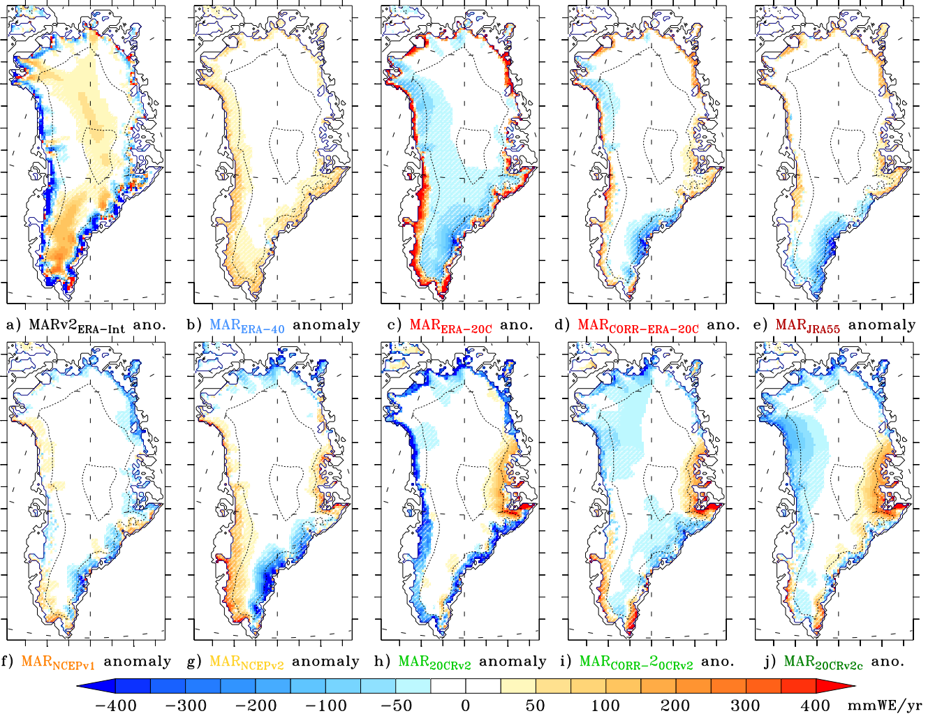
Figure 3. a) Difference between the mean annual SMB (in \text{mmWE mm w.e./yr} ) simulated by MARv2 forced by ERA-Interim and MARv3.5.2 forced by ERA-Interim over 1980–1999. b) Difference between the mean 1980–1999 annual SMB simulated by MARv3.5.2 forced by ERA-40 and simulated by MARv3.5.2 forced by ERA-Interim. c) Idem as b) but for ERA-20C. d) Idem as b) but for CORR-ERA-20c. e) Idem as b) but for JRA-55. f) Idem as b) but for NCEPv1. g) Idem as b) but for NCEPv2. h) Idem as b) but for 20CRv2. i) Idem as b) but for CORR-20CRv2. j) Idem as b) but for 20CRv2c. Finally, the areas where the differences are lower than the interannual variability of MARv3.5.2 forced by ERA-Interim over 1980–1999 are hatched.
