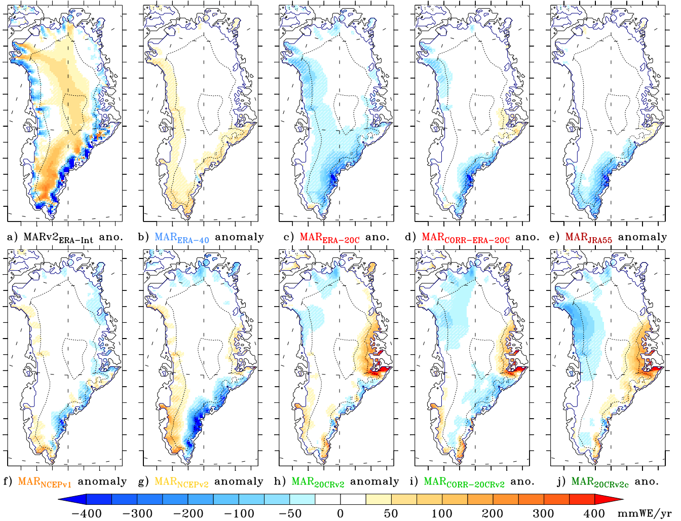
Figure 4. Same as Fig. 3 but for snowfall (in mmWE mm w.e. /yr).
