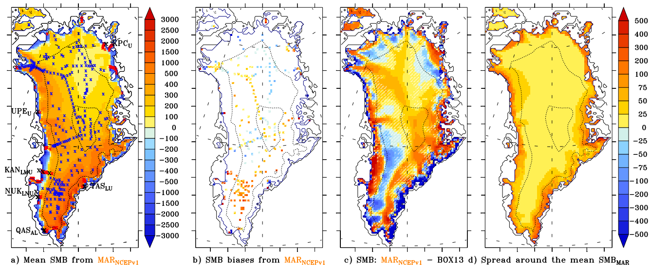
Figure 6. a) Mean annual SMB (in \text{mmWE/mm w.e./yr} ) simulated by MAR forced by NCEPv1 over 1958–2010. The ice core locations from Bales et al. (2001, 2009); Ohmura et al. (1999) used to validate MAR are quoted in blue while the MACHGUTH16 SMB sites (Machguth et al., 2016) are in red. b) Mean biases (in \text{mmWE/mm w.e./yr} ) of MAR forced by NCEPv1 over 1958–2010 with respect to both ice core and MACHGUTH16 based SMB estimations. The biases lower than the interannual variability of MARv3.5.2 forced by NCEPv1 over 1958–2010 are hatched. c) Comparison over 1958–2010 between the mean SMB (in \text{mmWE/mm w.e./yr} ) simulated by MAR and from the Box’s BOX13 reconstruction. Again, the biases lower than the interannual variability of MARv3.5.2 forced by NCEPv1 over 1958–2010 are hatched. d) Spread (i.e. standard deviation in \text{mmWE/mm w.e./yr} ) around 6 estimations of the mean 1958–2010 SMB as simulated by MAR forced by ERA, NCEPv1, JRA, CORR-ERA-20c, CORR-20CRv2, 20CRv2c.
