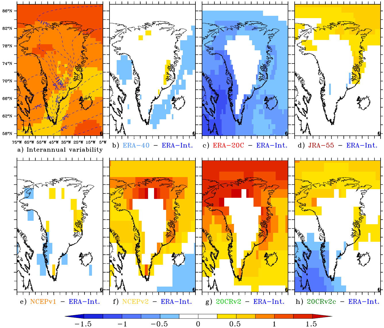
Figure 1. a) In background, the interannual variability (i.e. standard deviation) of the JJA mean 700 hPa temperature (T700) simulated by ERA-Interim over 1980-1999. Units are degrees Celsius. The contours of the mean JJA T700 is plotted in dashed blue. b)-h) Mean anomalies of the JJA 700 hPa temperature simulated by the different reanalyses used in this study with respect to ERA-Interim over 1980-1999 (in degrees Celsius). No comparison is shown above 2000m a.s.l. due to the aim of only showing comparisons in the free atmosphere (700hPa) only and the datasets are shown here by using their native Lat-Long projection. Similar figures over different reference periods and at other vertical levels (850 and 500hPa 500 hPa) can be found in the Supplementary Material.
