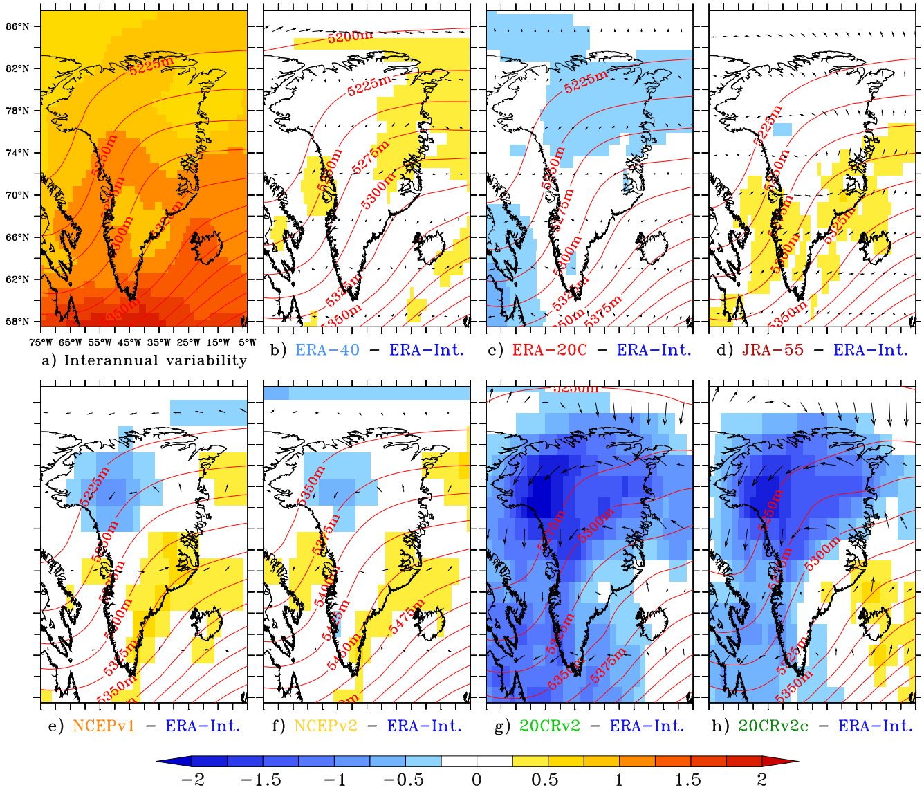
Figure 2. Idem as Fig. 2 but for the mean annual geopotential height (Z500) at 500hPa over 1980–1999. Units are meters. The wind vectors represent anomalies of wind field.
