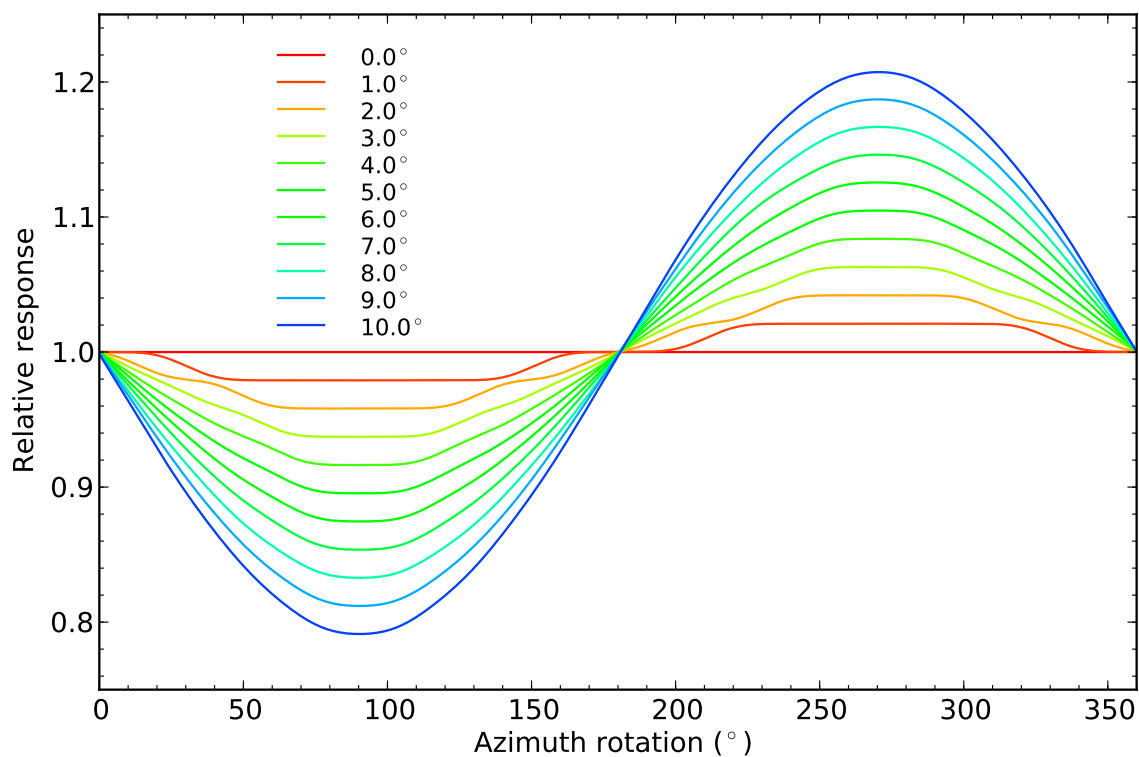
Figure 3. The relative response when tilting (various coloured curves) and rotating around azimuth an irradiance sensor on-board a platform 300 m above a snow surface. The solar zenith (azimuth) angle is 55.66^\circ ( 0^\circ ). The wavelength is 465 nm.
