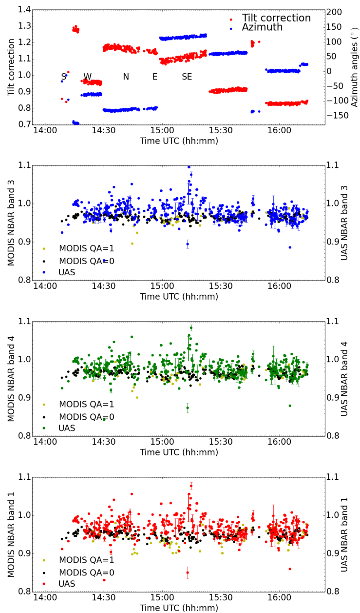
Figure 6. Top panel: The azimuth angle of the UAS (blue dots) and the tilt correction factor R^l/R^t , Eq. 3 (red dots). The various flight track elements are identified by letters and corresponds to the flight tracks in Fig. 2. Second-fourth panels: The MODIS (black=good quality and yellow=low quality dots) and UAS band 3 (blue), 4 (green) and 1 (red) NBARs as a function of time. In the case of several UAS data points within one MODIS pixel, the UAS data have been grouped together and presented as a dot with standard deviation. All data from the flight on Aug 6, 2010.
