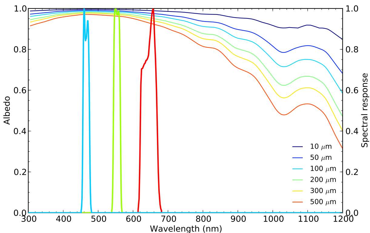
Figure 1. The pure snow albedo as a function of wavelength for snow grain sizes between 10-500 \mu\text{m} . Also shown in the thicker lines are the MODIS spectral response for band 3 (blue), 4 (green) and 1 (red). The spectral response data were obtained from http://mcst.gsfc.nasa.gov/calibration/parameters .
