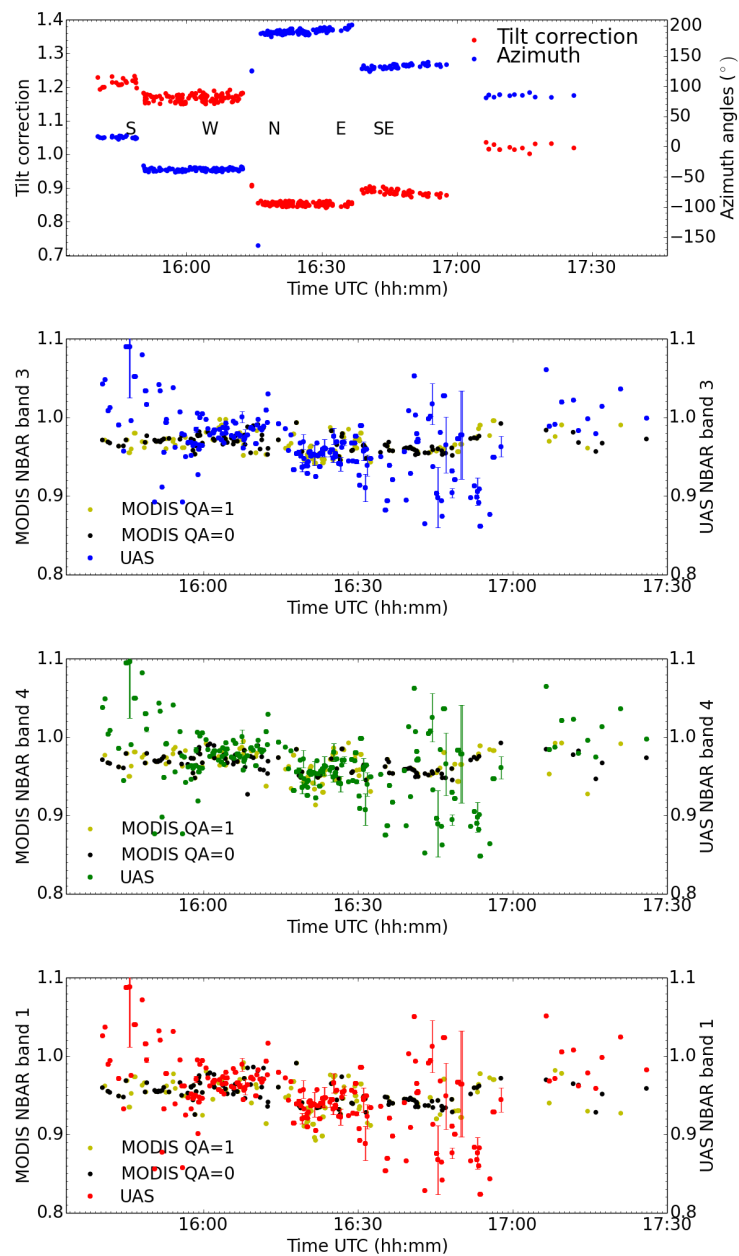
Figure 5. Top panel: The azimuth angle of the UAS (blue dots) and the tilt correction factor R^l/R^t , Eq. 3 (red dots). The various flight track elements are identified by letters and corresponds to the flight tracks in Fig. 2. Second-fourth panels: The MODIS (black=good quality and yellow=low quality dots) and UAS band 3 (blue), 4 (green) and 1 (red) NBARs as a function of time. In the case of several UAS data points within one MODIS pixel, the UAS data have been grouped together and presented as a dot with standard deviation. All data from the flight on Aug 5, 2010.
