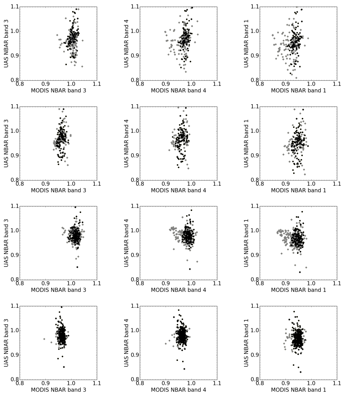
Figure 7. The MODIS (black=high quality and grey=low quality) versus UAS NBAR for bands 3, 4 and 1. Left column is data for band 3, middle column is band 4 data and right column is data for band 1. Rows 1 and 3 are MODIS version 5 and rows 2 and 4 MODIS version 6. Rows 1-2 (3-4) are data from the flight on Aug 5 (6).
