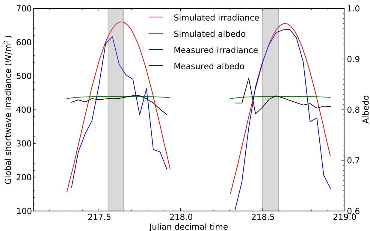
Figure 4. The measured (blue) and the simulated cloudless sky (red) downwelling short wave radiation for Summit, Greenland on Aug 5 (day 217) and 6 (day 218), 2010. The measured (black) and simulated (green) shortwave broadband albedos are also shown. The grey shaded areas indicate the time when the UAS was flying.
