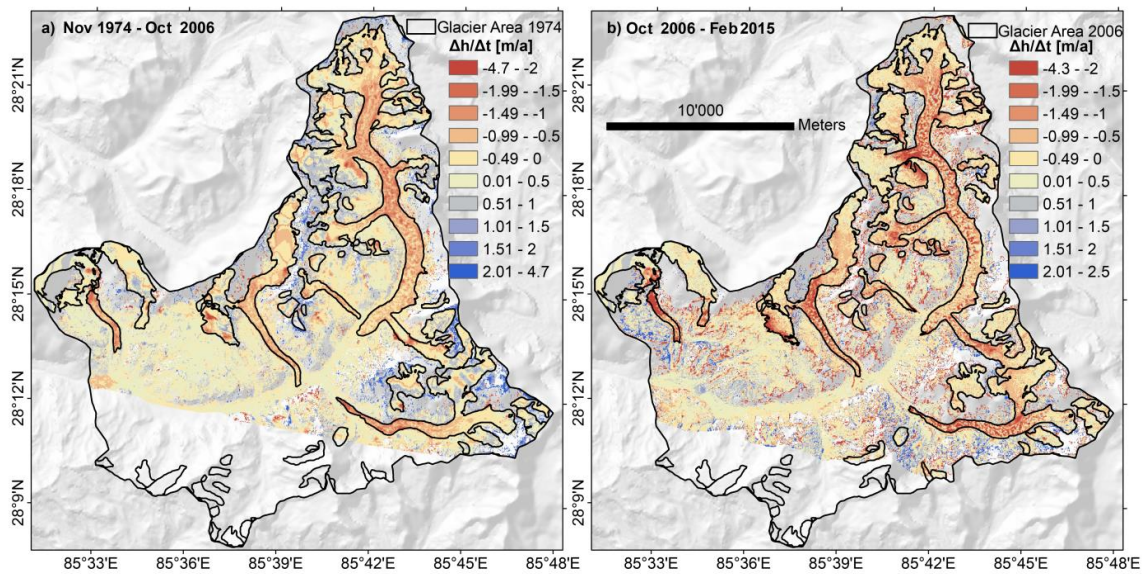
7 8 Figure 4. Elevation change rates ( \Delta h/\Delta t ) derived from a) Hexagon Nov 1974 and Cartosat-1 9 Oct 2006 DEMs and (b) Cartosat-1 Oct 2006 and WorldView Feb 2015 DEMs.
