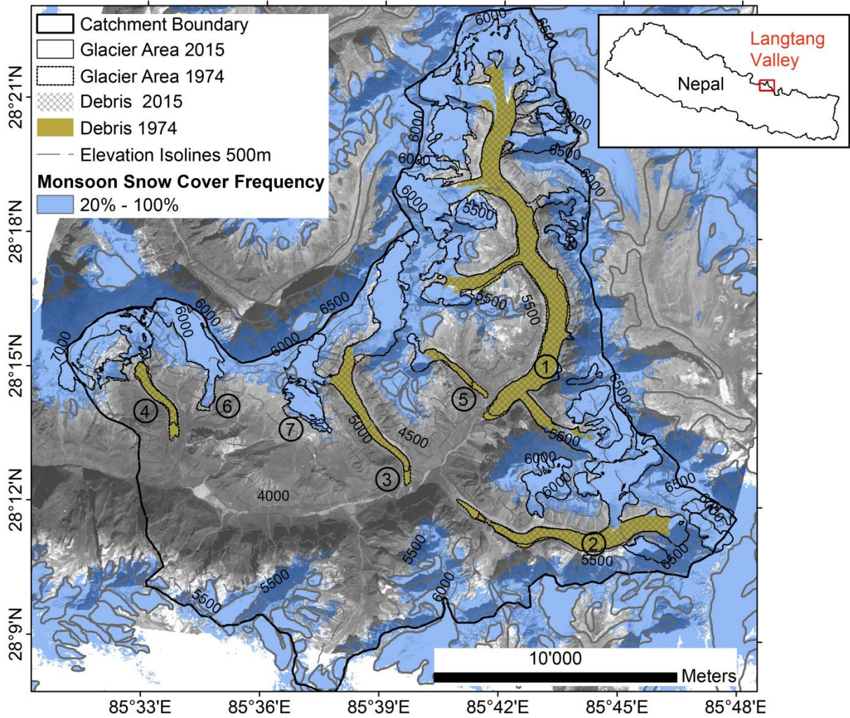
2 Figure 1. Map of the upper Langtang catchment. The numbers on the map correspond to the 3 glaciers listed in Table 1. Monsoon snow-cover frequency is based on Landsat 1999 to 2013 4 land cover classifications (Miles et al., 2016b). 1974 glacier area (dotted lines) is shown for 5 the seven studied glaciers only.
