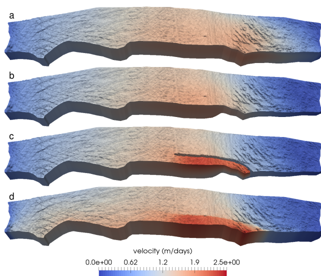
Figure 6. Magnitude of the modelled velocity field after the first (a), the second (b) and the third (c) optimisation, i.e. a) corresponds to the original setup with optimal parameters ( E, C, \alpha ) b) accounts for the optimal bump height on the bed while c) accounts for the optimal crack depth. For the sake of comparison, d) displays the measured UAV-inferred velocity field on the surface.
