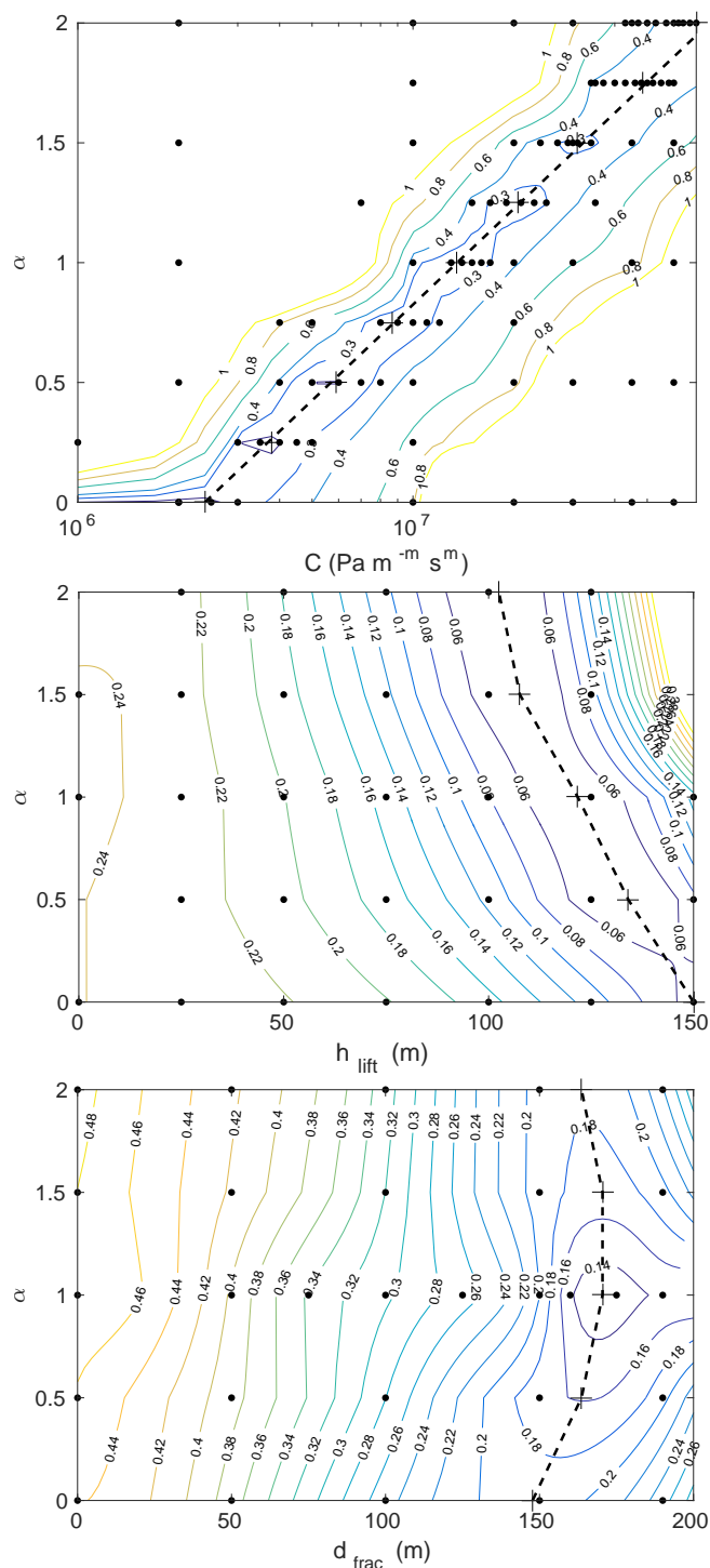
Figure 4. Level sets of the absolute misfit (in meters per day) between modelled and measured surface velocity magnitudes as function of parameters \alpha (Y axis) and C , h_{\text{lift}} , and d_{\text{frac}} (X axis), respectively. Each black dot corresponds to one model realization, from which the level sets were extrapolated. For each value of \alpha , the symbol + displays the minimum with respect to C , h_{\text{lift}} , or d_{\text{frac}} , respectively, while the dashed line connects + symbols.
