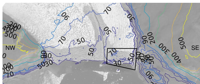
Figure 5. Contour lines of the Digital Elevation Model in the neighbourhood of the calving front. The polygon indicates the place where the bedrock was lifted in modelling experiments. The plot reveals the presence of a 20-meter-high bump on the glacier surface inside the polygon, and of a ridge on the south-east side of the glacier.
