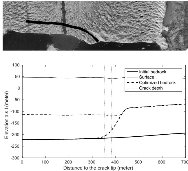
Figure 7. Top: Inferred position of the crack on the orthoimage of July 16. Bottom: Bedrock and ice surface along the main crack starting from the tip before and after optimizing the bump height and the crack depth to the UAV-inferred ice flow velocities. The dotted rectangle indicates the position where the crack crosses the moraine.
