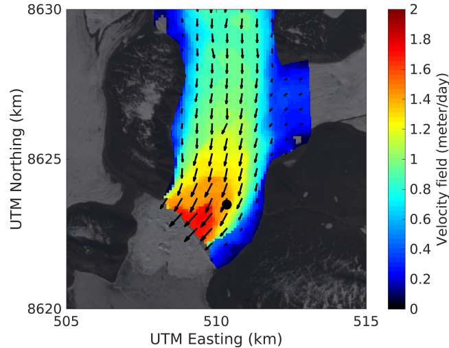
Figure 3. Average velocity field between June 14 and August 1 inferred by feature tracking from LANDSAT satellite images. The back dot indicates the position of the borehole.
