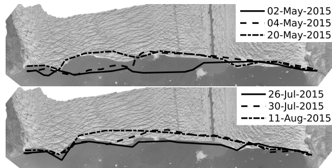
Figure 1. Positions of the calving front of Bowdoin Glacier inferred from satellite images before and after the calving events of May 3, May 19, July 27 and August 9.
