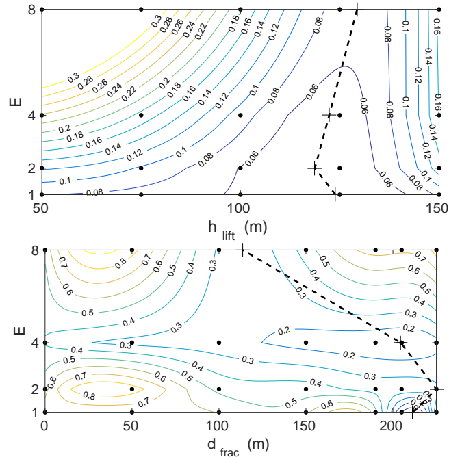
Figure 5. Level sets of the absolute misfit (in meters per day) between modelled and measured surface velocity magnitudes as function of parameters E (Y axis) and h_{\text{lift}} , and d_{\text{frac}} (X axis), respectively. Here, we used a constant parameter \alpha = 1 , and C was tuned to measured surface velocities in the extended model domain. Symbols have the same meaning as in Fig. 4.
