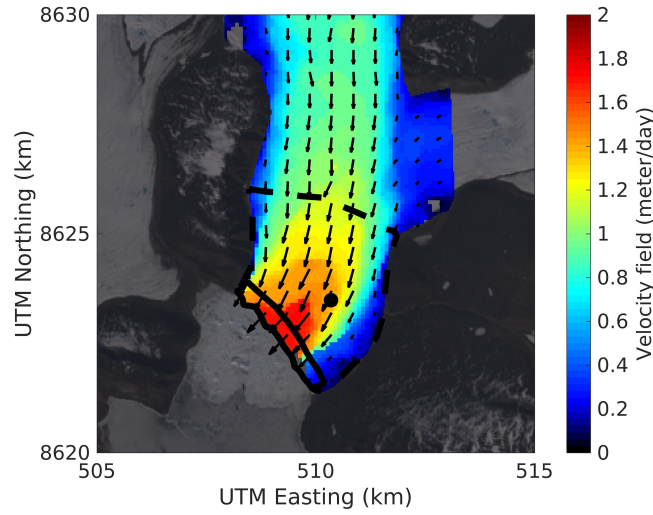
Figure 3. Average velocity field between June 14 and August 1 inferred by feature tracking from LANDSAT satellite images. The black dot indicates the position of the borehole. The dashed and continuous lines delimit the enlarged and reduced modelled domains, respectively.
