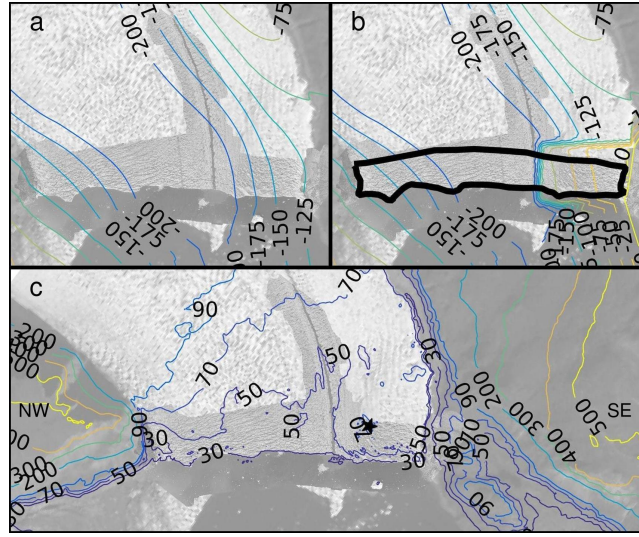
Figure 6. Contour lines of the initial bedrock topography (a), the optimized bedrock topography (b), and the digital elevation model (c) in the neighbourhood of the calving front. The thick line in panel b) indicates the reduced modelled domain, in which the bedrock was optimized. Panel c) reveals the presence of a 20-meter-high bump (materialized by symbol ★) on the glacier surface, and of a ridge on the south-east side of the glacier.
