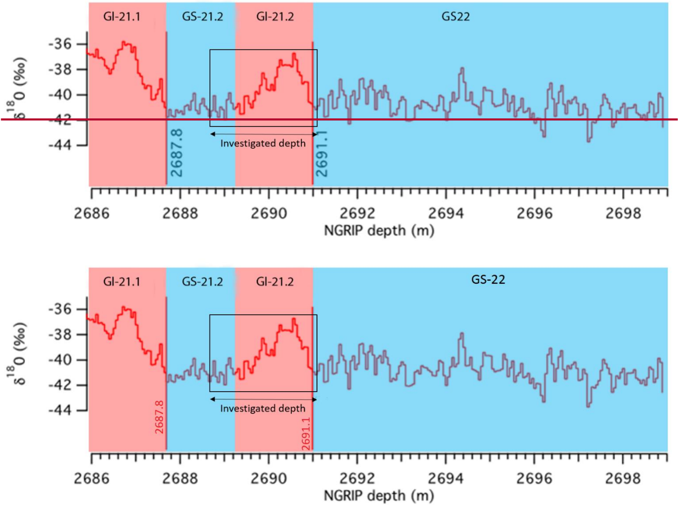
Figure 1: \delta^{18}\text{O} profile across the transition from GS-22 to GI-21.1 (modified from Vallelonga et al., 2012). Stadial and interstadial periods are highlighted in blue and red, respectively. The black box and arrow indicate the corresponding section of ice core analysed for this study.
