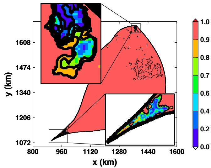
Figure 8. Stress ratio \zeta = \sqrt{\tau_{xz}^2 + \tau_{yz}^2} / \sigma_e computed for the constant-climate control run CTL with FS.
