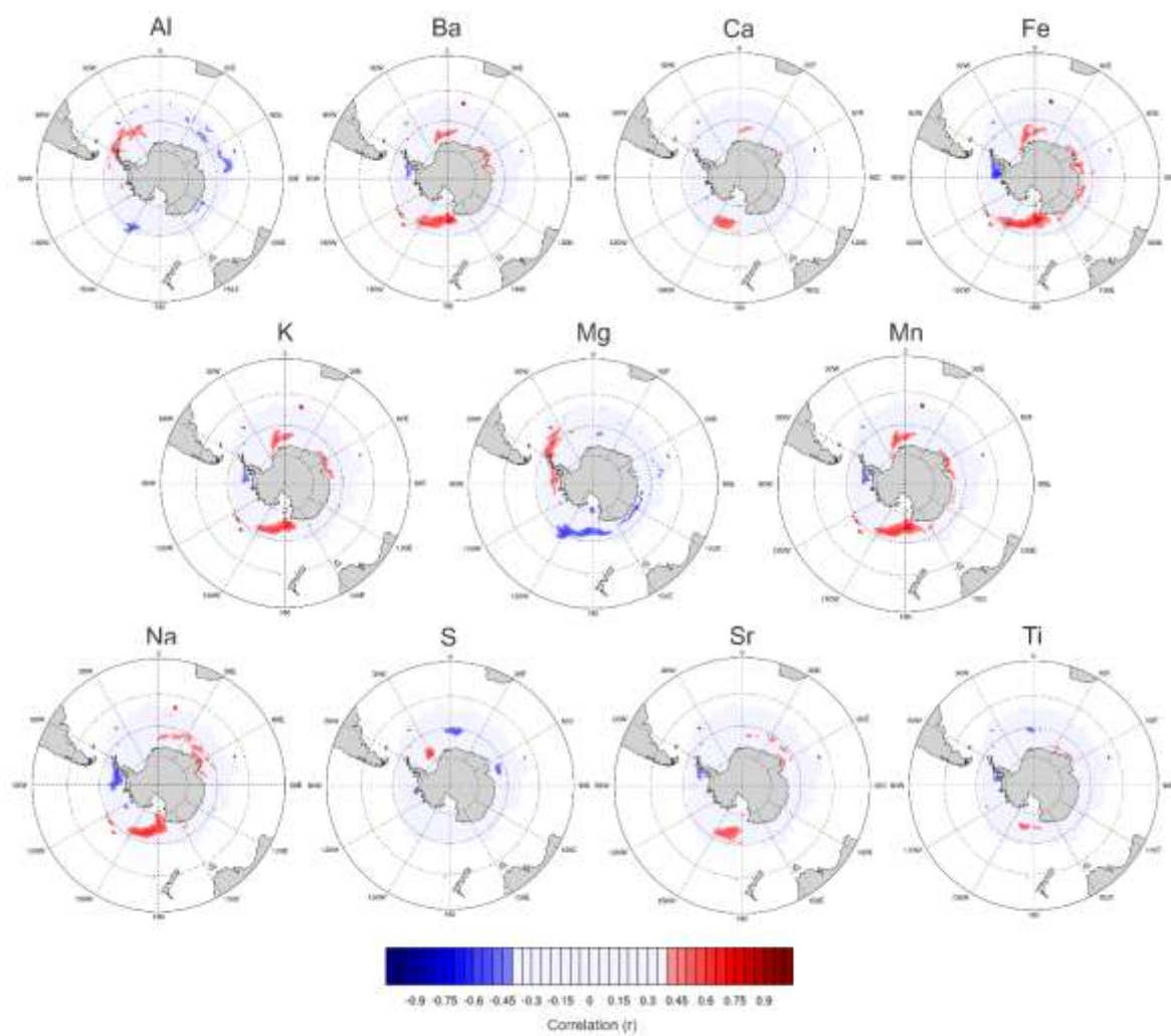
Figure 5: Correlation of the 1979–2008 ERA-Interim reanalysis sea ice concentration versus annually-averaged trace element time series in the MJ ice core.
