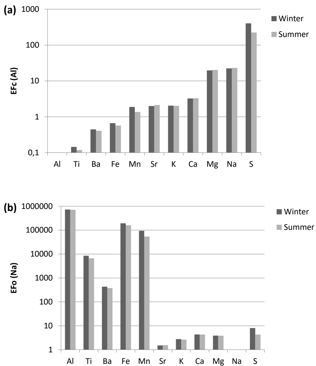
Figure 2. (a) Mean element enrichment factors in reference to Earth's crust (EF c ) and (b) oceanic composition (EF o ) at the MJ site for austral summer (December to February) and austral winter (June to August).
