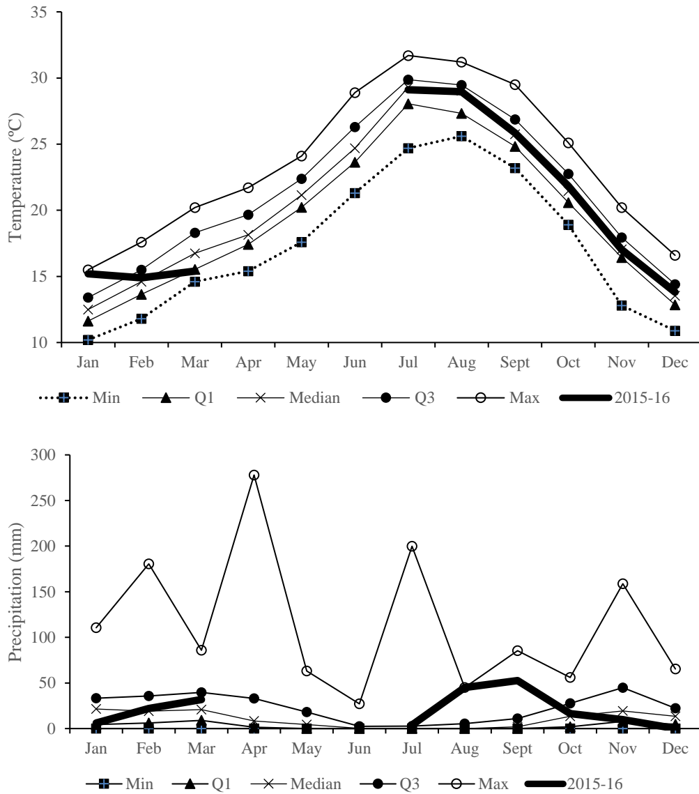
Figure 3: Statistics of monthly temperature and precipitation at Menara (Marrakesh) from 1977 to 2015 and records of the study period (July 2015 – March 2016). Source: NCDC/GHCN.
