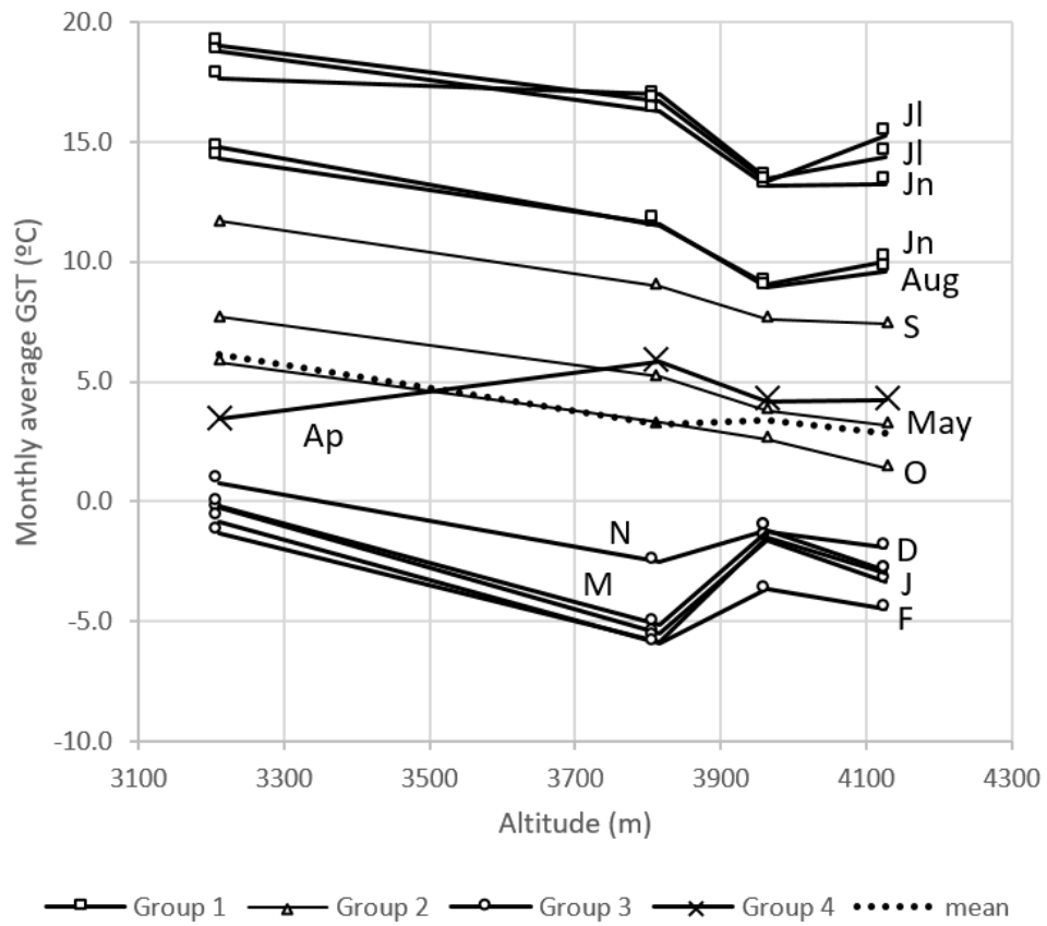
Figure 8: Mean monthly ground surface temperatures at the 4 study sites in the Toubkal Massif from July 2015 to June 2016.
