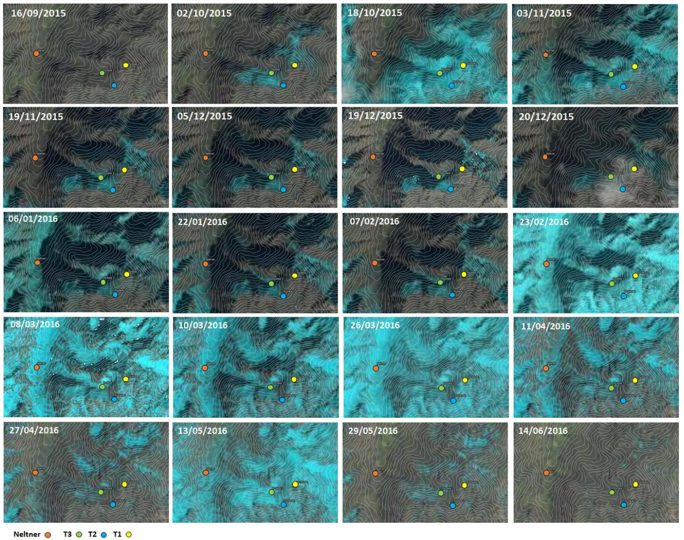
Figure 5: Satellite true colour composite scenes from Landsat-8 (USGS) and Sentinel-2 (ESA) used for assessing the snow cover at the monitoring sites from September 2015 to June 2016. Light blue indicates snow cover and brown and green indicate snow free terrain. Satellite imagery obtained from USGS EarthExplorer.
