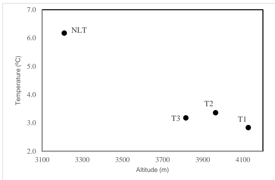
Figure 7: Mean annual ground surface temperatures vs altitude for the 4 monitored sites in the Djebel Toubkal massif.
