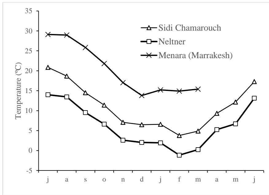
Figure 4: Mean monthly air temperatures from July 2015 to June 2016 in Marrakesh (Menara), in the two study sites and extrapolated to the summit of Djebel Toubkal (4,167 m a.s.l.).
