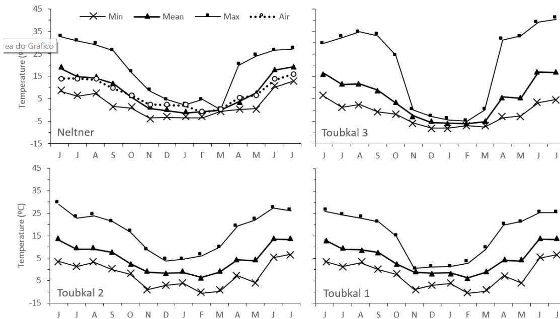
Figure 6: Monthly ground surface and air temperatures in the Djebel Toubkal massif from June 2015 to July 2016. Extremes are absolute monthly maximum and minimum temperatures.
