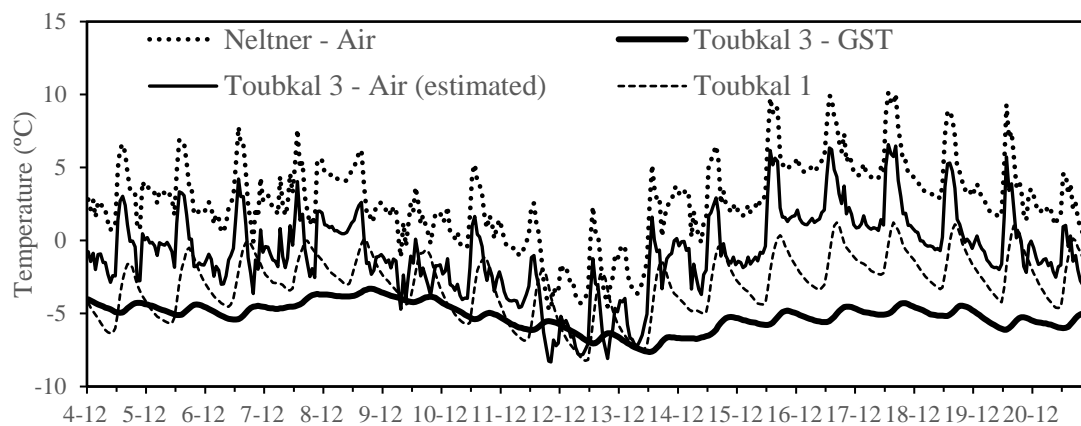
Figure 10: Example of the hourly GST regime at Toubkal 3 and comparison with air temperatures measured at Neltner and extrapolated to T3 using the observed lapse rate of -0.59^{\circ}\text{C} \cdot 100\text{ m}^{-1} .
