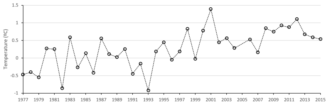
Figure 14: Estimated mean annual air temperatures at the summit of Djebel Toubkal (4,167 m asl) obtained from extrapolation of temperatures from Menara (Marrakesh) using a lapse rate of -0.59^{\circ}\text{C} \cdot 100 \text{ m}^{-1} .
