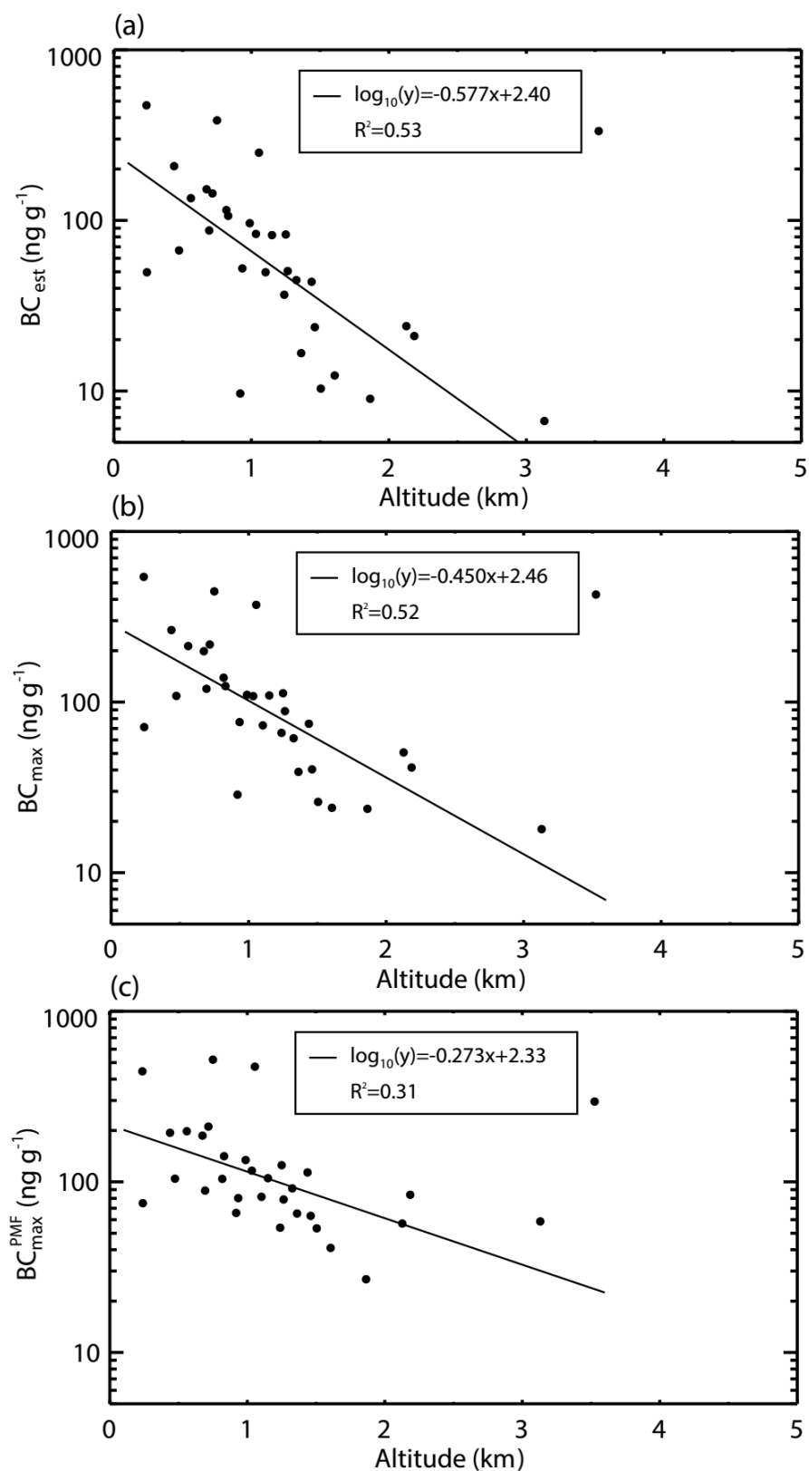
Fig. 8. (a) C_{BC}^{\text{est}} and (b) C_{BC}^{\text{max}} measured according to the ISSW and (c) C_{BC}^{\text{max, PMF}} determined by the PMF model for the surface snow for each site as a function of altitude for the sites in Xinjiang.
