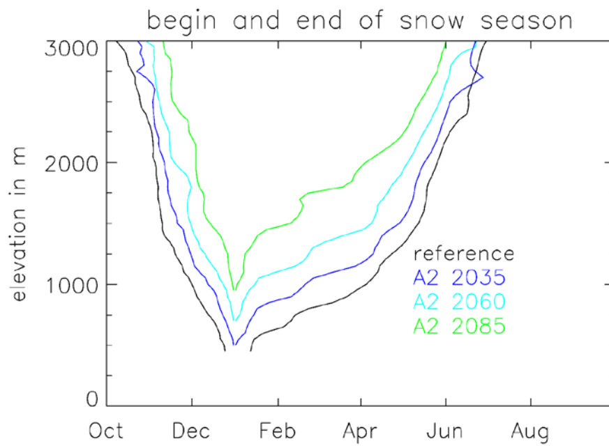
Figure 7: Begin and end of a continuous snow cover for the A2 emission scenarios for the reference and three future time periods in the Aare region.
