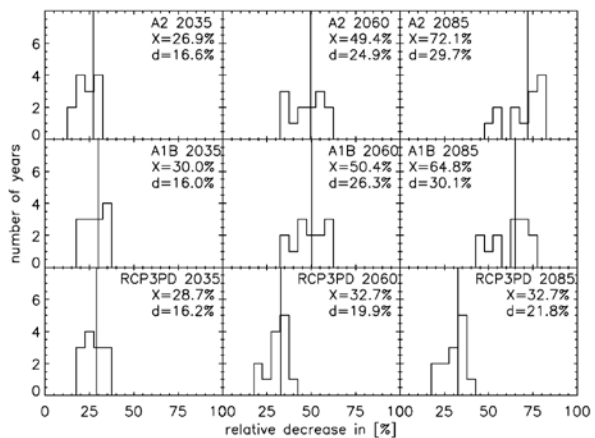
Figure S2: Distribution of the annual relative decreases of the snow depth for A2, A1B and RCP3PD and the three different future time periods (2020-49, 2045-74, 2070-99) for Aare (top) and Grisons (bottom) based on the inter-annual variability of the reference period. The value X corresponds to the spatial and temporal mean relative decrease in [%], which is visualized in Figure 3. The value d defines the difference between the highest and the lowest relative decrease within the scenario period. The number of the simulated years is N=13.
