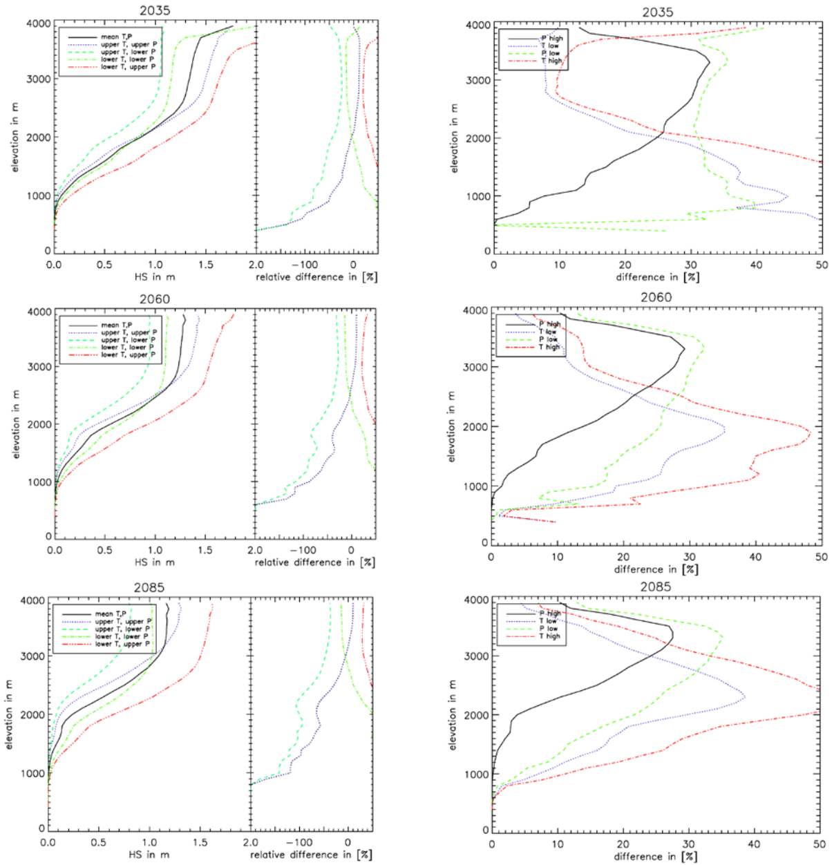
Figure S6: Elevation dependence of absolute snow depth for five possible T-P combinations (left) and decrease relative to the mean T, mean P configuration (left panels). Elevation dependence of the relative snow depth difference (%) for four different combinations T-P (right panels). "T high" means the difference of the upper T - lower T at the upper P configuration. "P low" means the difference of the upper P - lower P at the lower T configuration. This is shown for 2035 (top), 2060 (middle) and 2085 (bottom) based on the A2 emission scenario in the Aare region.
