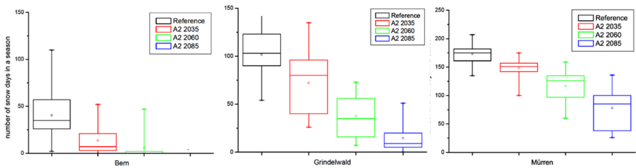
Figure 8: Inter-annual variability of the number of snow days (snow depth at least 5 cm) at three stations (Bern 540 m (left), Grindelwald 1030 m (center) and Mürren 1650 m (right)) in the Aare region. The little square in the box plots represents the mean value and the whiskers show the 2.5 % and 97.5 % quantile value of the different model simulations.
