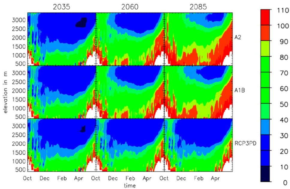
Figure 5: Relative decrease (%) of the snow depth in the Aare region for the three emission scenarios (top, middle, bottom) and the three different time periods (left to right) dependent on season and elevation. The white colors indicate no data.
