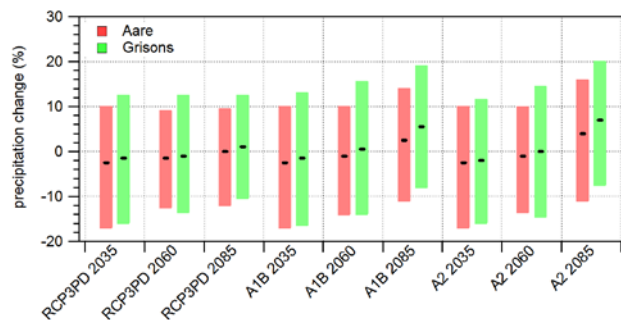
Figure 2: Mean January to March temperature (left) and precipitation (right) changes including the uncertainty bars from the upper and lower estimates for the Aare (red) and the Grisons (green) region.
