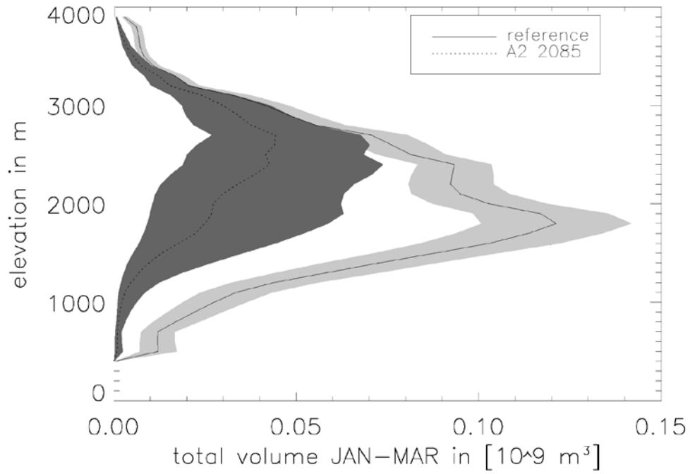
Figure 6: Total volume of snow (Jan-Mar) in the Aare region for the today (solid line) and the end of the century (dotted line). The shaded area for the reference period indicates half of the standard deviation (for readability) of the inter-annual variability. The shaded area of the 2085 scenario period indicates the range between the lowest and highest estimate based on the A2 emission scenario (Table 3).
