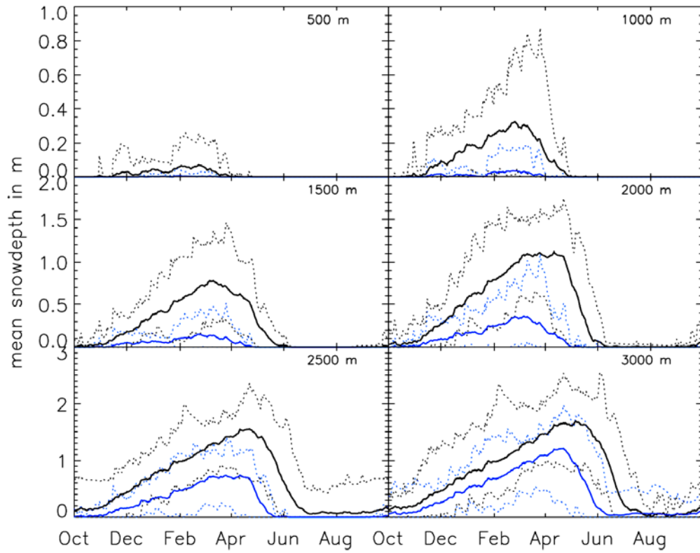
Figure 4: Mean (solid), maximum and minimum (dotted) snow depth for the reference period (black) and the A2 2085 scenario (blue) in the Aare domain for 6 elevation zones. The elevation zones are 100 m wide, i.e. the 1500 m zone, contains all pixels between 1450 and 1550 m. Note: the scale of the y-axis changes with elevation.
