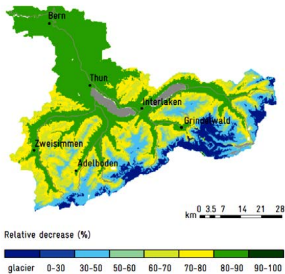
Figure S3: Relative decrease for February 1 snow depth of during the last time period (2085) and the A1B scenario for the Aare region (left) and the Grisons region (right).
