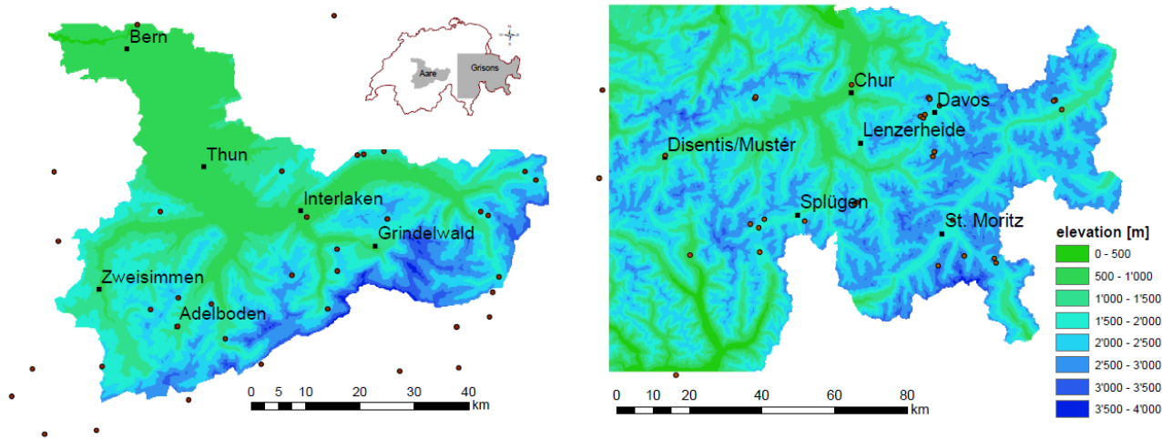
Figure 1: Elevations of in the Aare (left) and the Grisons region (right). Weather stations used for simulations are marked with dots. The location of the two regions within Switzerland is given shown by in the red inset with the two grey areas.
