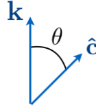
Figure 2. In a single crystal, the sound velocities depend only on \theta .
