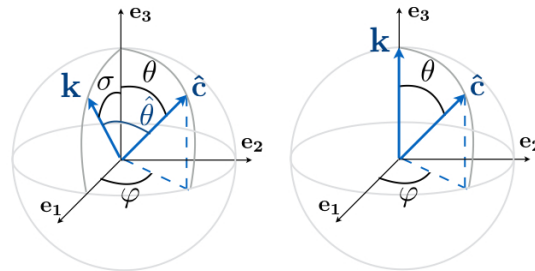
Figure 7. (a) System of angles used in Bennett's calculations. \hat{c} is given by (\varphi, \theta) and \mathbf{k} is given by \sigma , being otherwise in the (\mathbf{e}_1, \mathbf{e}_3) plane. The extra angle \hat{\theta} denotes the angle between \mathbf{k} and \hat{c} , thus \cos \hat{\theta} = \sin \sigma \cos \varphi \sin \theta + \cos \sigma \cos \theta . (b) Particular case of the Bennett configuration, for \sigma = 0 ; in this case, \hat{\theta} = \theta .
