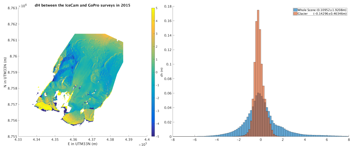
Figure 10. DEM differences between simultaneous IceCam and GoPro surveys of 2015. Residual doming is evident in the GoPro survey, as well as areas where either the IceCam or the GoPro surveys failed to produce useful data because of a lack of texture in the images (fresh snow, for instance). A histogram of the differences, after removal of outliers ( dH > 10m ), is shown to the right for the whole scene and for the glacier only.
