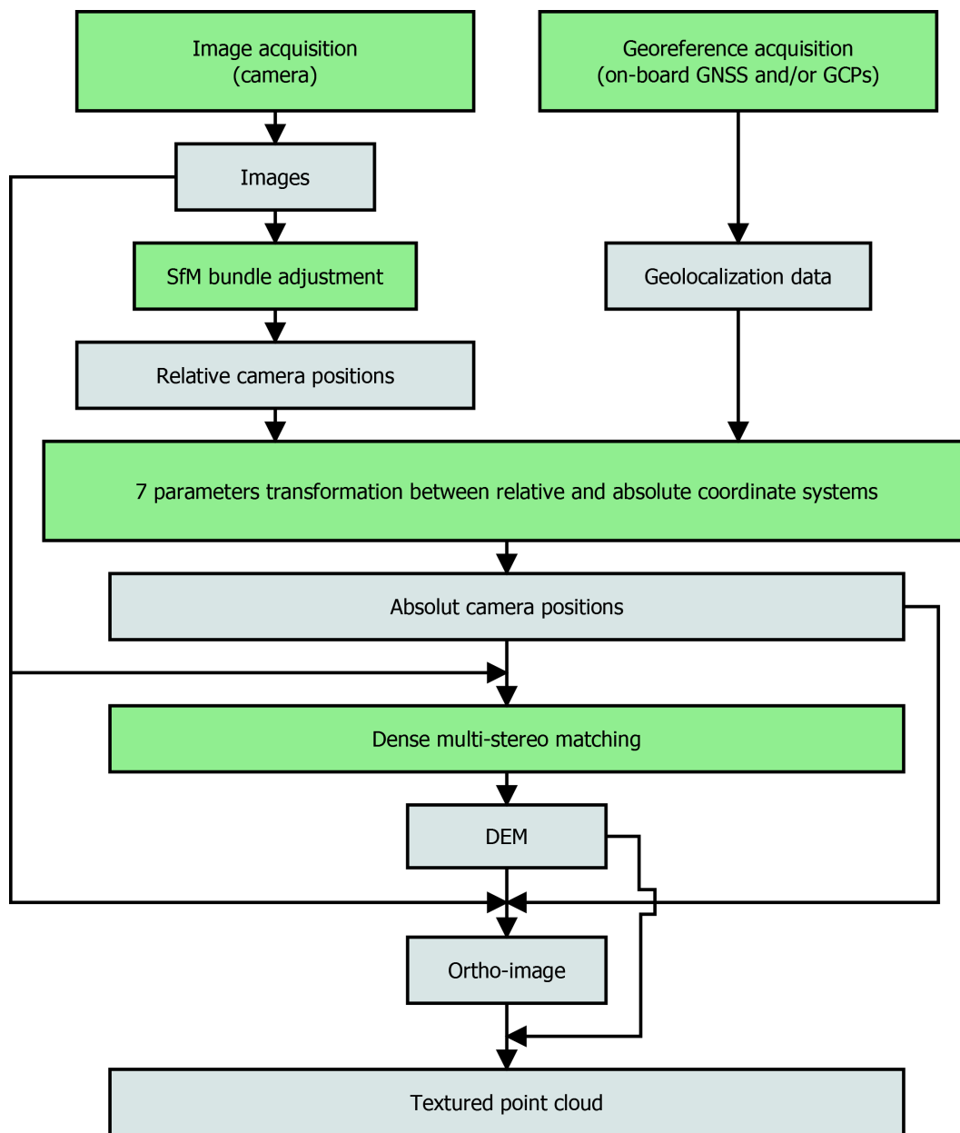
Figure 1. Standard SfM Photogrammetry processing workflow. Green boxes are processes and grey boxes are products.
