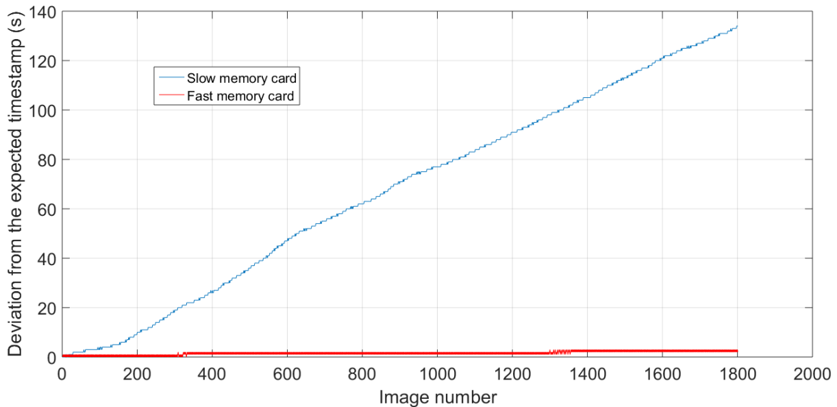
Figure 3. Differences between expected time stamps of pictures for a 30-minute period with a lapse time of one second and the EXIF time stamp recovered from the first 1800 images of a GoProH3+BE. Results are either for a relatively slow micro-SD card (64GB SanDisk Ultra microSDXC Class 10 UHS-I) or a fast card (32GB SanDisk Extrem Plus microSDHC UHS-I/U3). The fast card diverges by only 2s after 30 minutes, while the slow card diverges by 134s at a visibly irregular rate.
