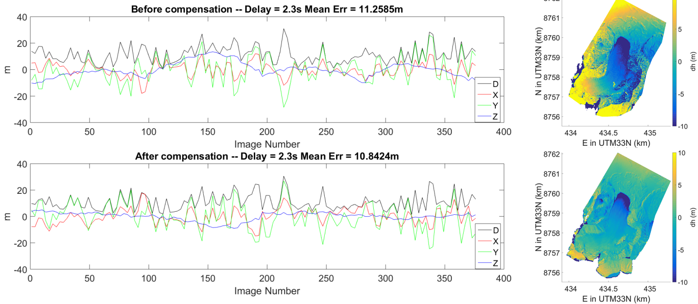
Figure 7. Residuals of the fit between the GNSS-extracted positions and the relative SfM-based orientation of the images, before and after the GNSS-guided bundle adjustment for the 2015 flight. There is a systematic error in the z-axis coming from a misestimated focal length (each of the 4 ”bumps” in the blue line representing the residuals in the z-axis in the upper panel corresponds to a line of flight (Figure 9)). Right-hand panels show the DEM differences to a reference DEM from 2010. The non-compensated DEM (upper-right panel) has a significantly stronger dome-shaped distortion pattern. After correction, the magnitude of the doming is less than the precision of the GPS.
