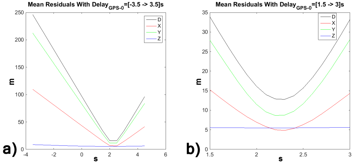
Figure 2. Mean residuals in x, y and z and Cartesian distance D of differences between raw GPS positions and SfM-reconstructed relative positions, as a function of different start-time Delay_{GPS-Camera_0} offsets between GPS and camera. a) search area from -3.5 to +3.5 s, in 0.5-s increments; b) finer-scale are from 1.5 to 3.0 s in 0.1-s increments. The best value is found at \approx Delay_{GPS-0} = 2.3s . Note that the z coordinate is nearly independent of Delay_{GPS-Camera_0} , because the flight used here was mostly at a constant altitude.
