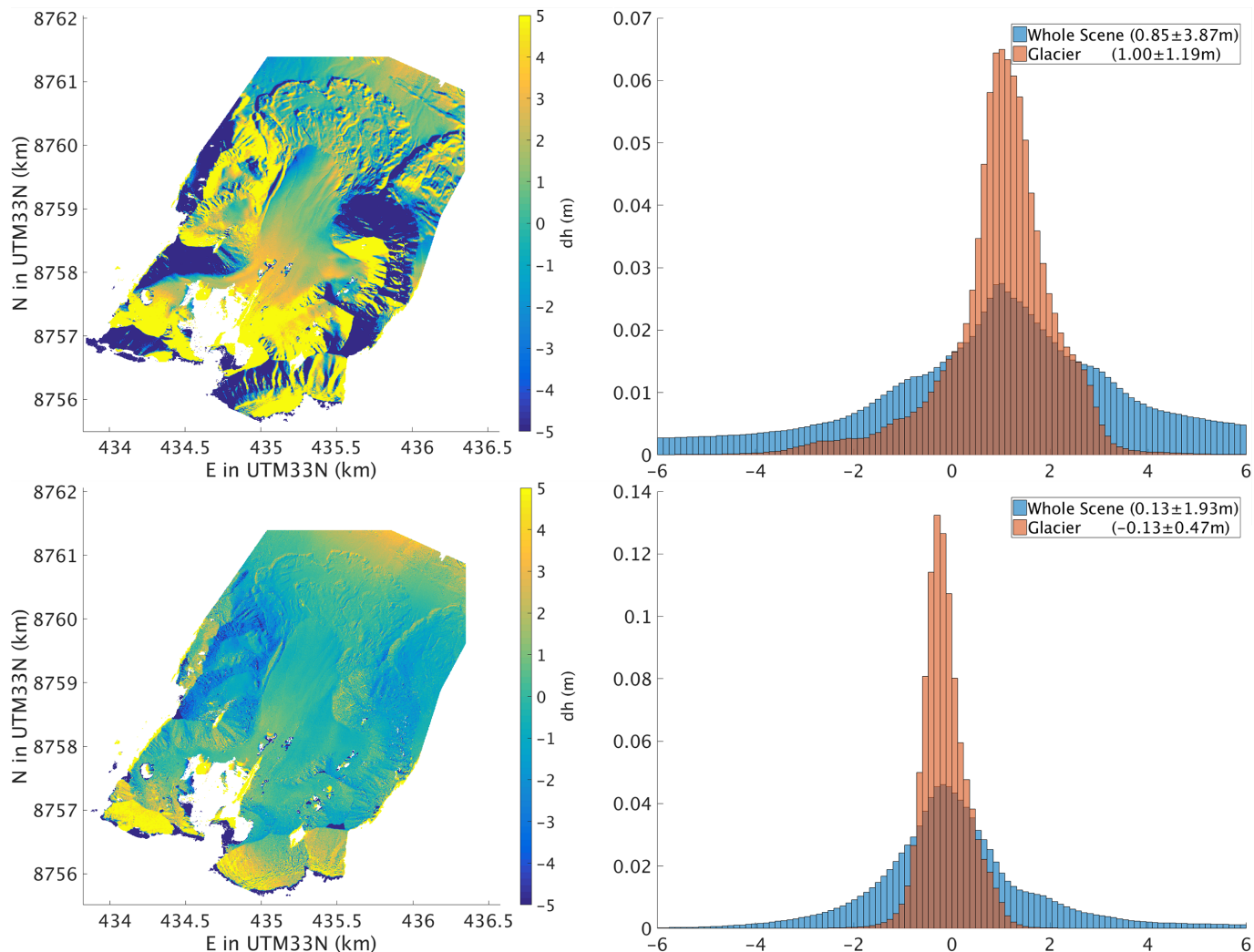
Figure 10. DEM differences between simultaneous IceCam and GoPro surveys of 2015. Top row without refined camera times, bottom row with refinements. Residual doming is evident even in the refined GoPro survey, as well as areas where either the IceCam or the GoPro surveys failed to produce useful data because of a lack of texture in the images (fresh snow, for instance). Histograms of the differences, after removal of outliers ( dH > 10m ), is shown to the right for the whole scene and for the glacier only.
