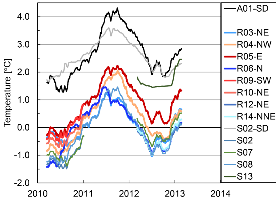
Figure 5. Mean annual rock- and soil surface temperatures (all except A01-SD) and air temperature (A01-SD) during the period Sept. 2009 to Aug. 2013 shown as simple moving 365-days average for all sites. To ensure that the temperature variability was not shifted in time, the mean values were centered (an equal number of days on either side of the mean value). A01-SD is air temperature in Signaldalen (SD), R03 to R14 are the rock face loggers and S02 to S13 are the soil temperature loggers.
