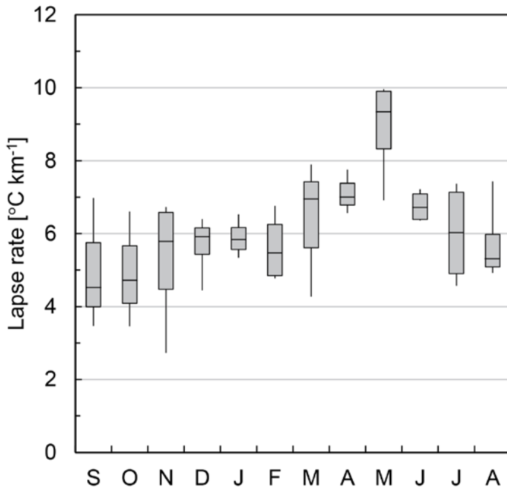
Figure 9. Inter-annual variability from 2009-2013 in monthly-mean lapse rates based on air temperature data from Rihpojavi (502 m asl) and Signaldalen (65 m asl) from 2009-2013. Boxes show the interquartile range of the month's lapse rate, horizontal lines inside the boxes show the median values, and the whiskers show the full range of the data.
