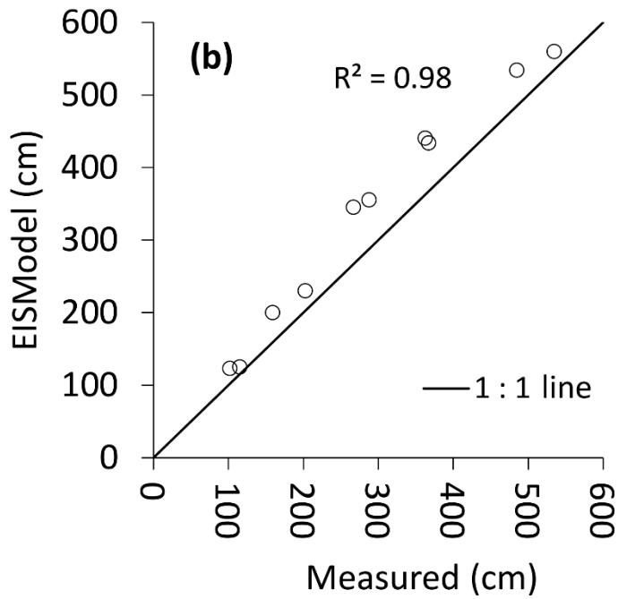
Figure 3 Mass balance modelled by EISModel compared with a) pollen dating in the period from 2005 to 2009, and b) mass balance measurements in the validation period from 2009 to 2013.
