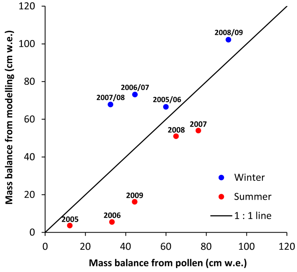
5 Figure 5 Comparison of the winter and summer mass balance as obtained by pollen dating and modelling (EISModel).
