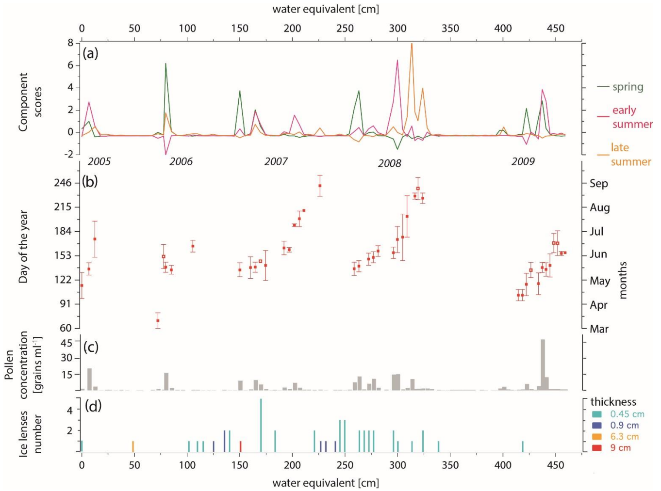
5 Figure 2 (a) Mt. Ortles firn core 2009 timescale (Festi et al., 2015) based on Principal Component Analyses. As every principal component (PC) condenses the seasonal information of the pollen spectrum, scores values should be interpreted as follows: a sample (w.e. depth down) presenting high component scores values for a specific PC is characterized by a pollen content reflecting predominantly the season corresponding to that particular PC. (b) Mean date (day of the year \pm 1 sigma) obtained by using the new method developed in this paper; empty squares represent inversions (c) Pollen concentration in the Mt. Ortles 2009 firn core. (d) Number and mean thickness (colour scale) of ice lenses per sample.
