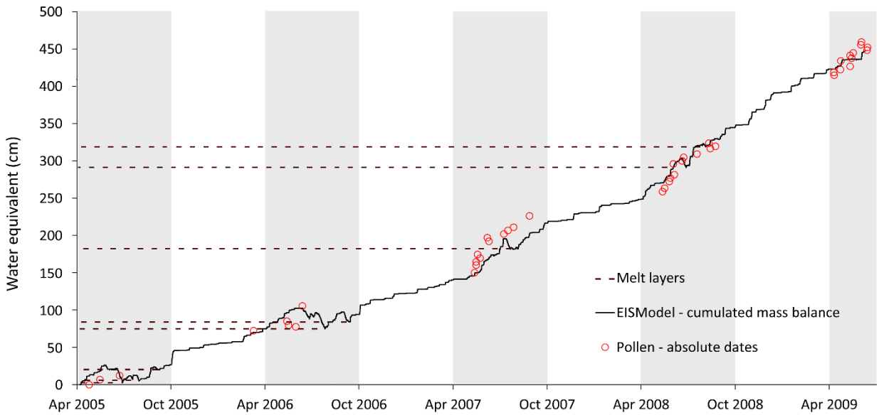
Figure 4 Comparison between cumulated mass balance modelled by EISModel and obtained by pollen dating. Alternating grey/white bars have a six months duration and roughly indicate the warm/cold season. Horizontal dash lines indicate melt layers.
