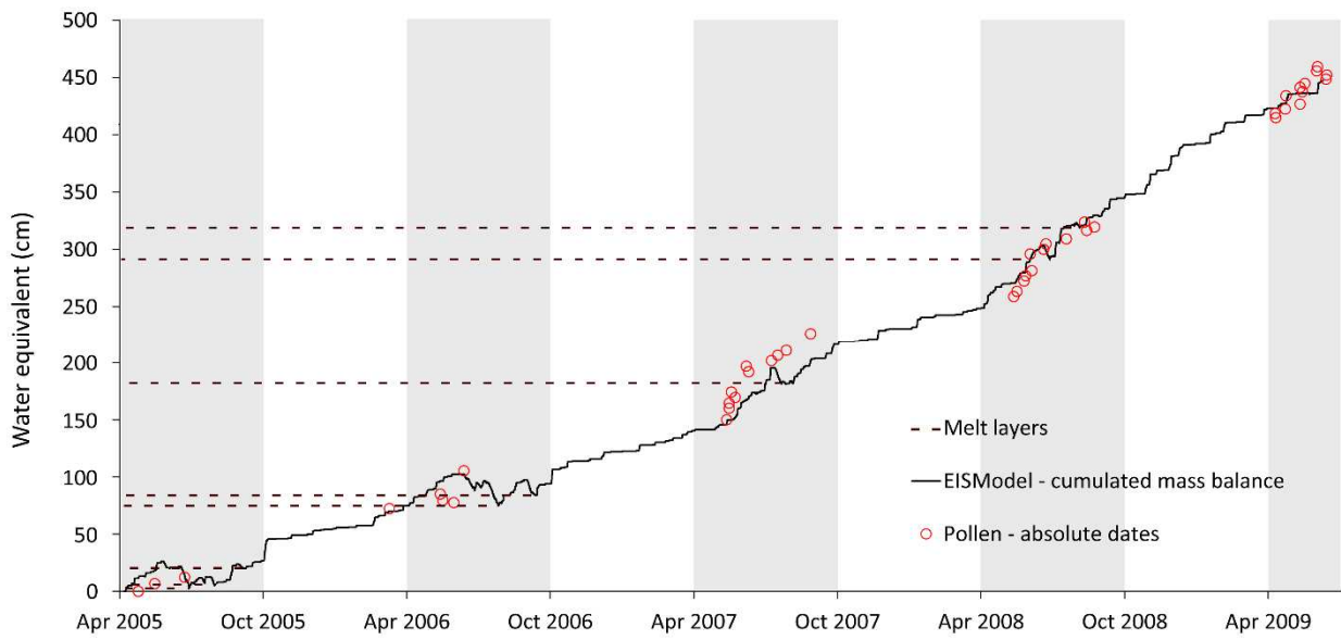
Figure 3-4 Comparison between cumulated mass balance modelled by EISModel and obtained by pollen dating. Alternating grey/white bars have a six months duration and roughly indicate the warm/cold season. Horizontal dash lines indicate melt layers.
