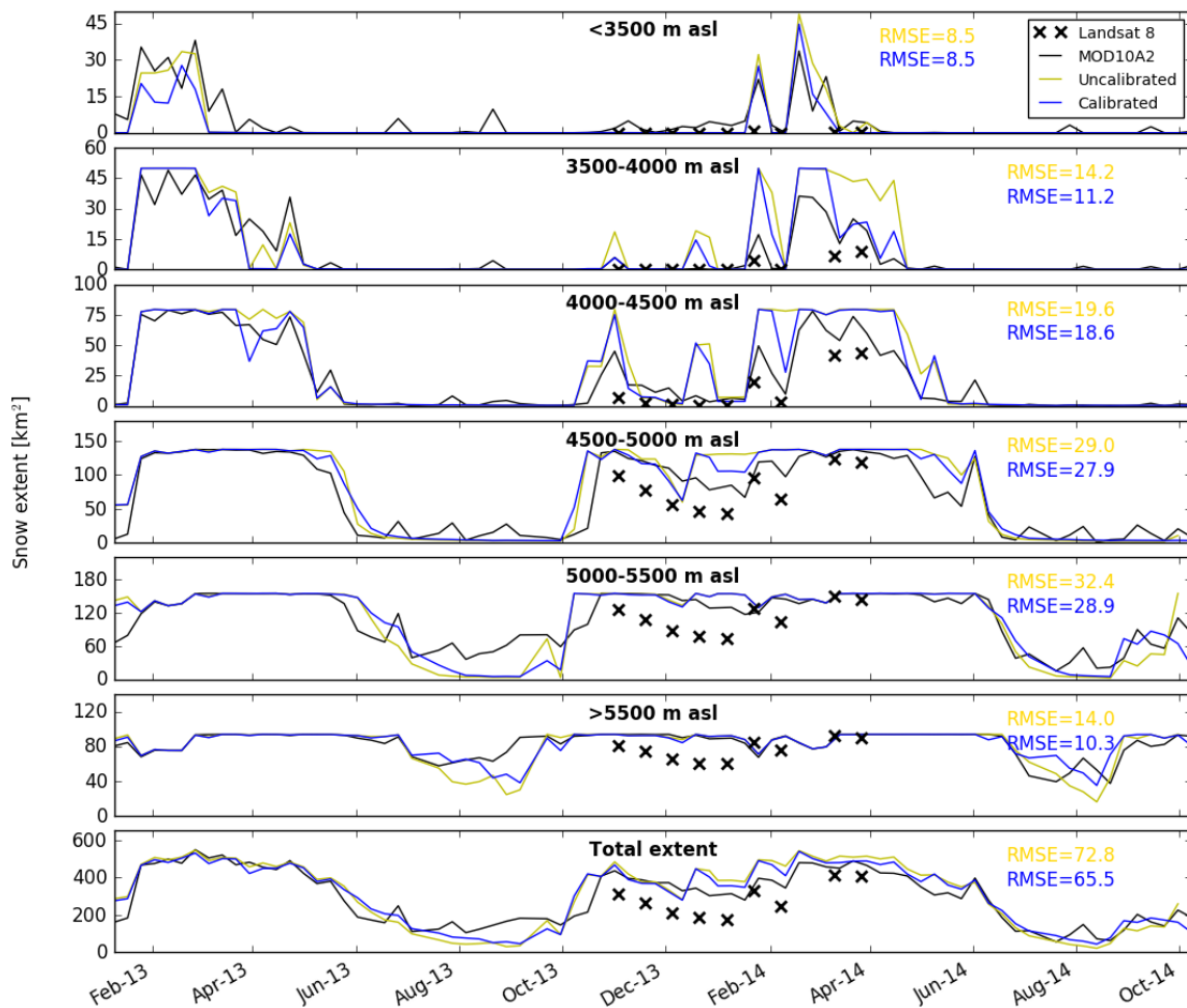
Figure 4: Modelled 8-day maximum snow extent before and after calibration (ensemble mean), Landsat 8 snow extent and MOD10A2 snow extent per elevation zone. The RMSE (km²) is given per zone for the fit between modelled (before and after calibration) and MOD10A2 snow extent.
