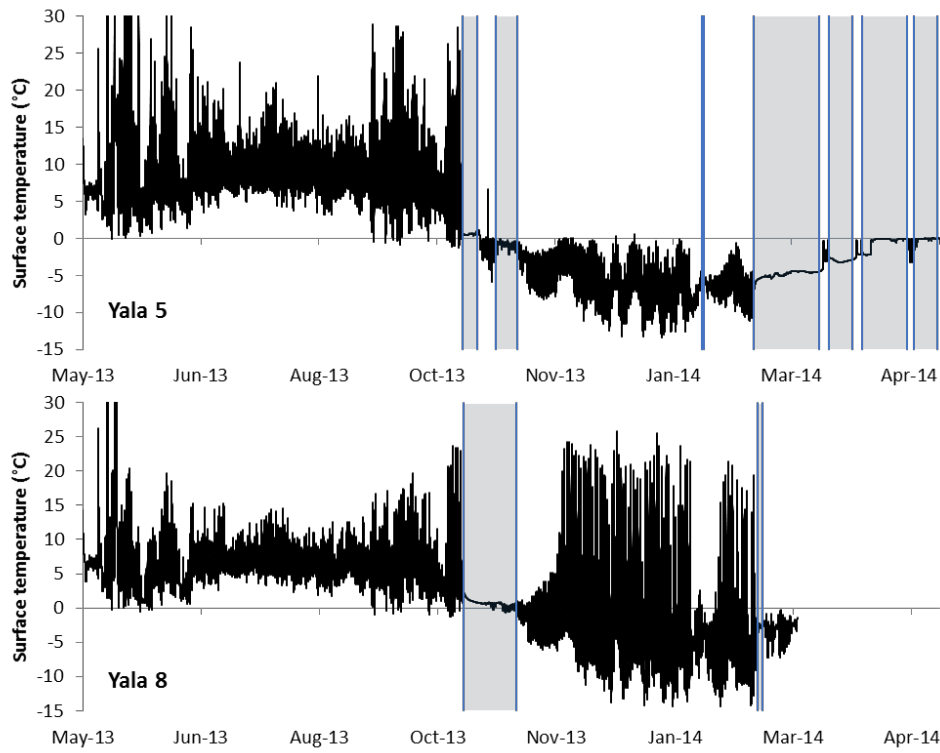
Figure 2: Observed surface temperature with 10 minute interval at two locations. The blue vertical lines indicate the start and end of the snow cover.
