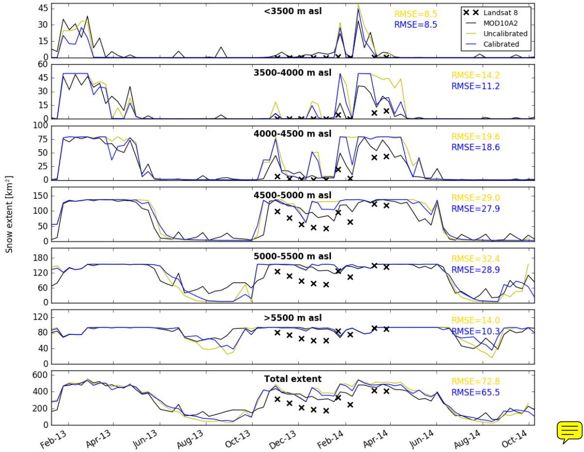
5 Figure 3: Modelled 8-day maximum snow extent before and after calibration (ensemble mean), Landsat 8 snow extent and MOD10A2 snow extent per elevation zone. The RMSE (km 2 ) is given per zone for the fit between modelled (before and after calibration) and MOD10A2 snow extent.
