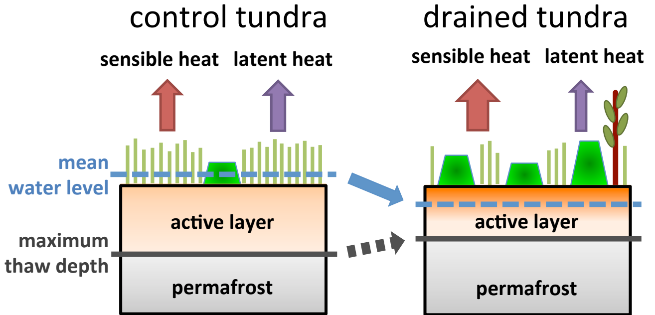
Figure 10: Expected changes in growing season properties of a tundra ecosystem as response to drainage disturbance.
