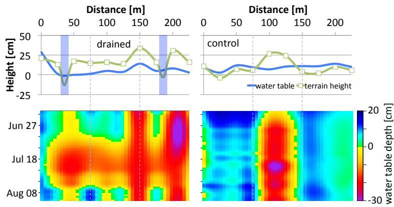
5 | Figure 4: Top panels: Variability of terrain height (green lines, boxes indicating microsite study positions) and water table depth (blue lines) along transects in the drained (left) and control (right) sections of the observation site (water table depth reflects conditions in mid July 2014). Blue shading in drained panel indicates position of drainage channel, where interpolation of terrain height was modified. The zero level was chosen arbitrarily, so absolute heights do not carry any information in the top panels; bottom panels: Development of water table depth over time for the period Jun 18 to Aug 14, 2014 (interpolated over both space and time). Values are given relative to the surface, with negative values indicating water tables below the surface level.
