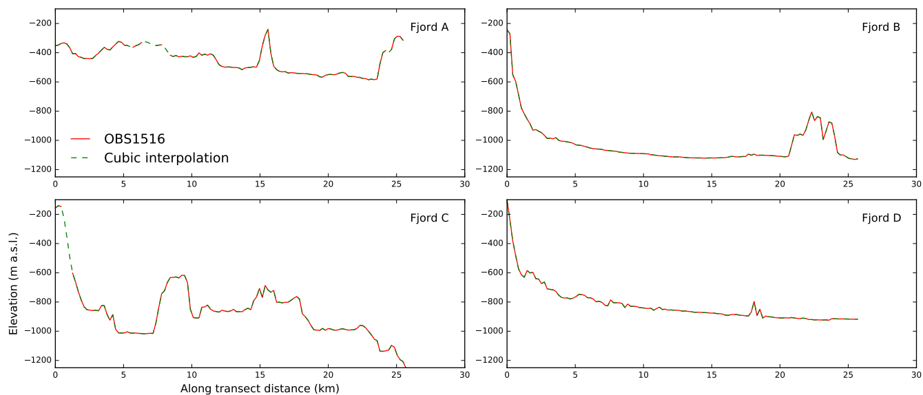
Figure 8. Examples of the along-transect profile of four fjords from the area of interest depicted and labelled in Fig. 7(a) and 7b respectively. Along-transect distance starts at the head of each fjord and extends to the fjord mouth.
