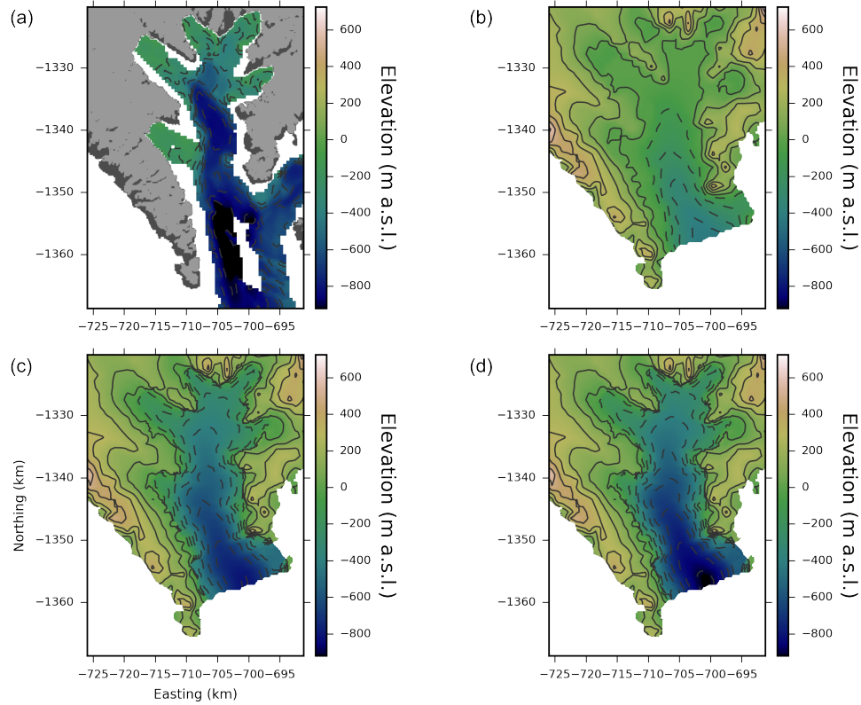
Figure 9. The area of interest close to Cape York displaying (a) the land mask of the area of interest (Morlighem et al., 2014) with the extent of OBS1516 in grey with ice (light grey), ice-free land (dark grey) and ocean (white) along with the OBS1516 elevations, (b) Bed2013 elevation, (c) Bed2013 combined with the SynthIBCAO synthetic geometry and (d) Bed2013 with the inclusion of the SynthOBS synthetic geometry. SynthIBCAO and SynthOBS are only used within the ocean regions of the land mask.
