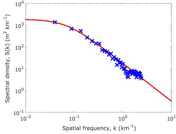
Figure 13. Composite power spectral density from fjord bed elevation profiles. Blue crosses indicate spectral data that has been averaged over nine fjord profiles, and the solid red curve is the best fit to the parametric model, equation 3.
