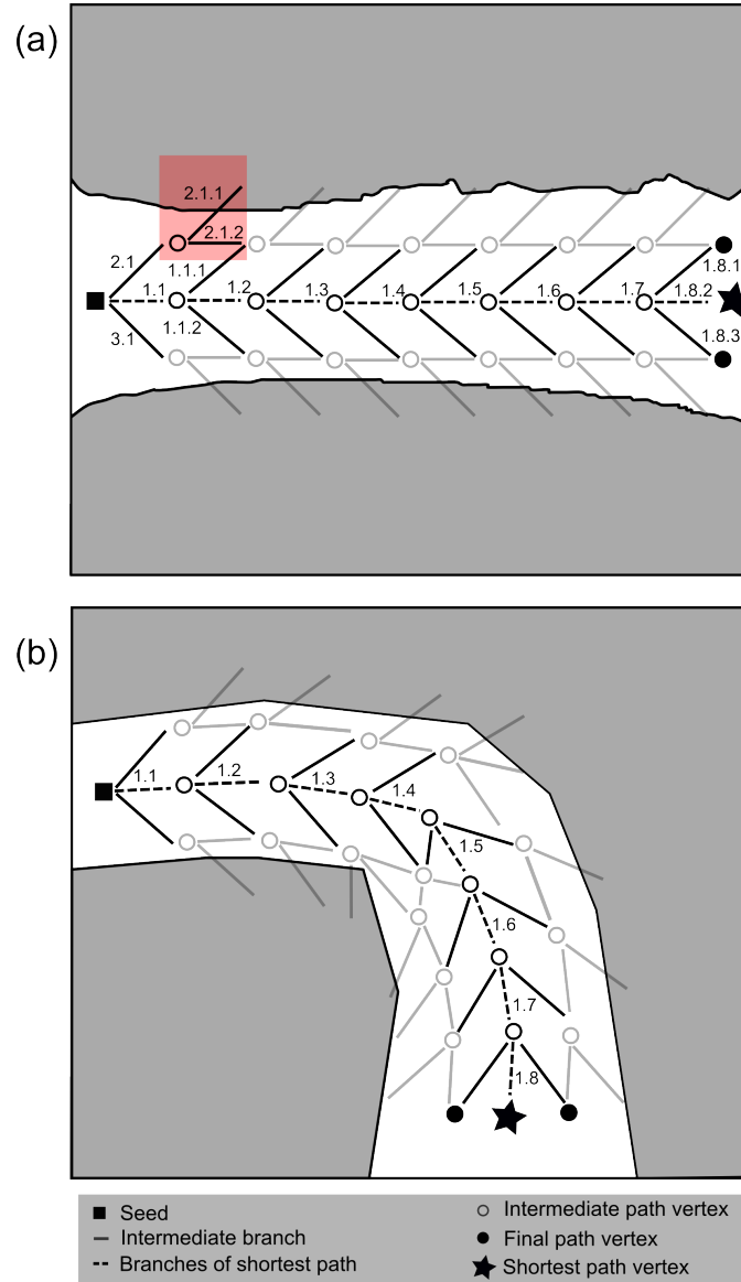
Figure 5. Fjord-centrelines approach where (a) fjords are identified from the GIMP land-classification mask (Morlighem et al., 2014) as being sections of ocean between land/ice regions (b) An example of the centrelines-pathfinder algorithm as applied to a single fjord. From a seed point, children are spawned, each time resulting in the creation of new branches. Where children intersect the land/ice boundary, branches are culled. The culling of branches 2.1.1 and 2.1.2 within the pink box, as well as the selection of the shortest path is discussed in the text. Please refer to the online version of this article to make use of references to colour. Generalisation of the fjord centrelines approach where the centrelines-pathfinder algorithm is applied to a (a) straight ford and (b) a curved fjord. From a seed point, children are spawned, each time resulting in the creation of new branches. Where children intersect the land/ice boundary, branches are culled. The culling of branches 2.1.1 and 2.1.2 within the pink box in (a), and the selection of the shortest path is discussed in the text.
