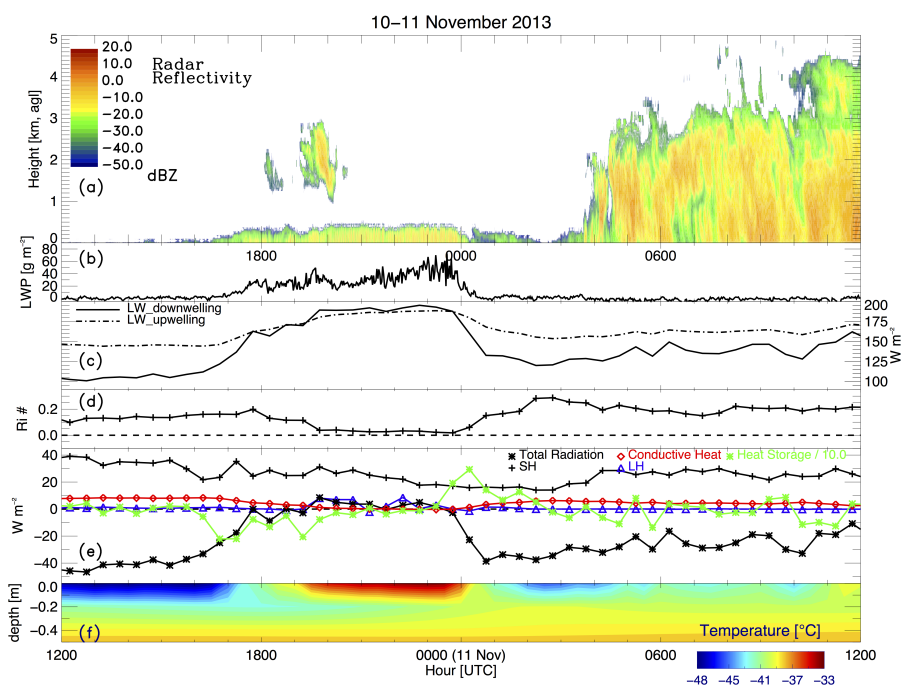
Figure 2. A case study from 12 UTC on 10 November 2013 to 12 UTC on 11 November 2013. (a) Cloud occurrence as seen by the MMR, (b) liquid water path, (c) longwave upwelling and downwelling radiation, (d) Richardson number, (e) surface energy fluxes: total radiation, sensible heat, latent heat, conductive heat and heat storage/10.0 and (f) subsurface temperatures.
