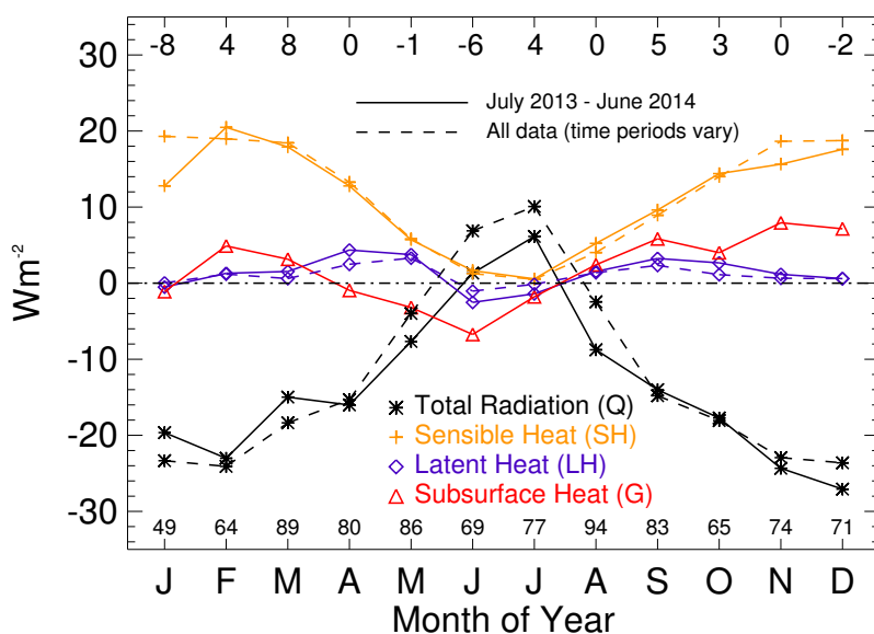
Figure 4. Monthly mean values of the 4 SEB terms for the period July 2013 – June 2014. The values at the top of the figure are the monthly residual of the SEB ( \text{W m}^{-2} ). The values at the bottom of the figure are the percentage of the month for which all 4 SEB terms are available.
