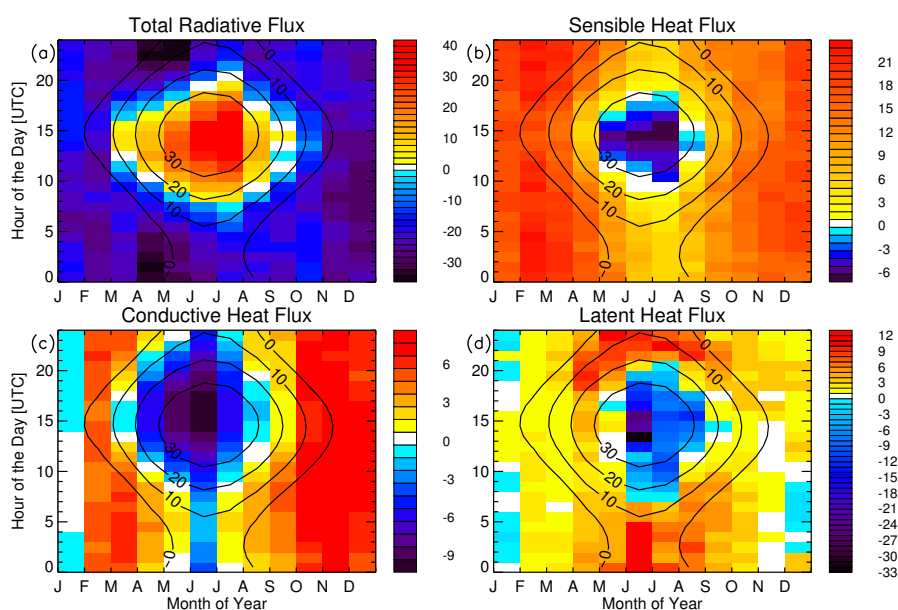
Figure 5. Monthly-hourly mean values from July 2013 – June 2014 of (a) total radiative flux, (b) sensible heat flux, (c) conductive heat flux and (d) latent heat flux. Black contour lines indicate the solar elevation angle. Units on the color bars are all in \text{W m}^{-2} .
