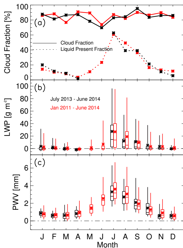
Figure 6. a) Cloud fraction (solid) and liquid present fraction (dotted, \text{LWP} > 5 \text{ g m}^{-2} ), b) liquid water path and c) precipitable water vapor. Statistics shown in black (red) are for available data spanning July 2013 – June 2014 (January 2011 – June 2014). Distributions are represented by box-and-whisker plots (the box indicates the 25th and 75th percentiles, the whiskers indicate 5th and 95th percentiles, the middle line is the median, and the * is the mean).
