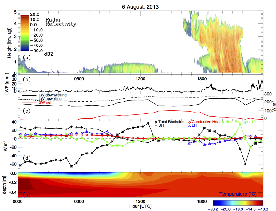
Figure 3. A case study on 6 August. (a) Cloud occurrence as seen by the MMCR, (b) liquid water path, (c) longwave upwelling, longwave downwelling, and net shortwave radiation, (d) surface energy fluxes: total radiation, sensible heat, conductive heat and heat storage/10.0 and (e) subsurface temperatures.
