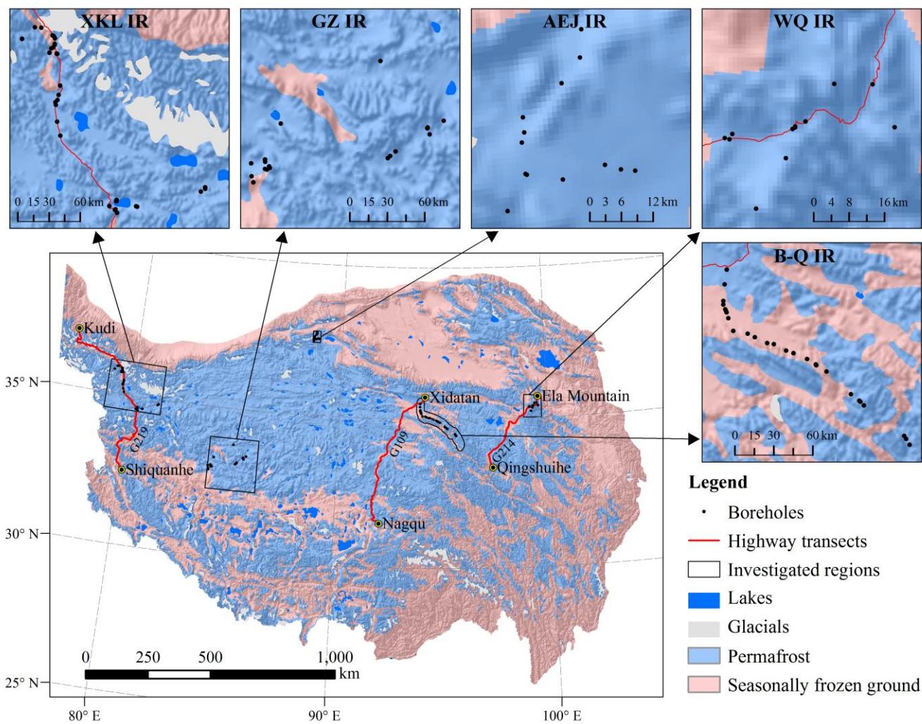
695 Figure 1. Spatial distribution of the field survey regions on the Tibetan Plateau (based on the permafrost distribution map made in 1996)
