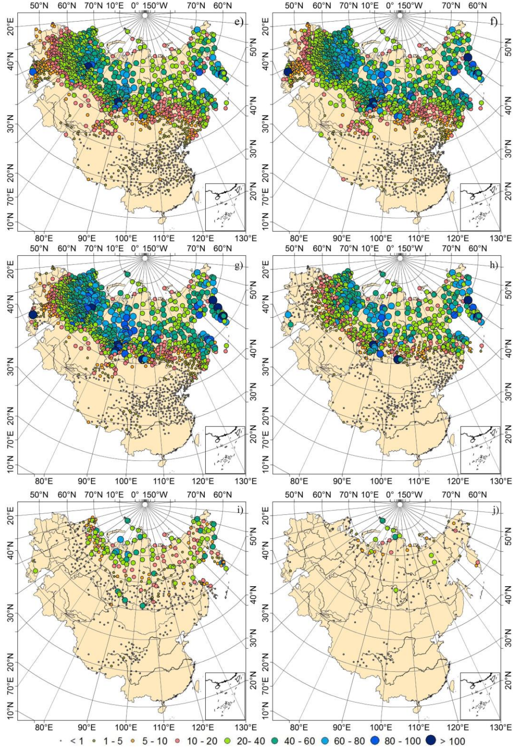
1 2 Figure 3. Monthly mean snow depth (from September to June) (cm) across the Eurasian continent 3 (cm) during 1966-2012. (a) September, (b) October, (c) November, (d) December, (e) January, (f) 4 February, (g) March, (h) April, (i) May, (j) June.
