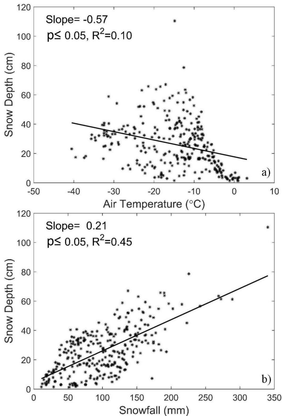
Figure 9. Relationship between long-term mean annual mean snow depth and air temperature (a) and between long-term mean annual snow depth and snowfall (b) from 386 stations from November through March during 19661971-2009-2000 over the USSR. The thick line is a linear regression trend.
