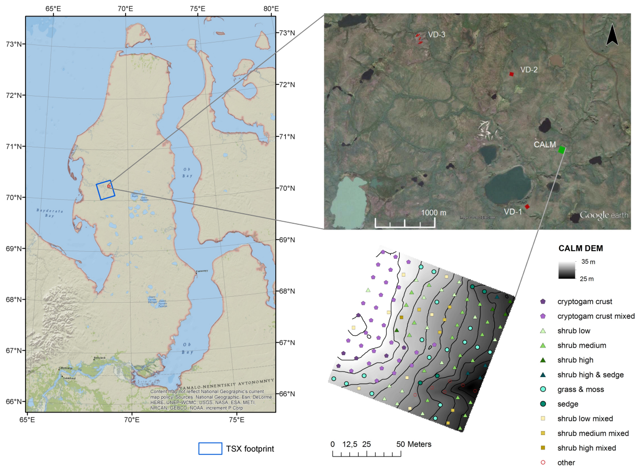
Figure 1. Location of the study area ( with monitoring sites Vaskiny Dachi (VD) 1-3 and CALM grid ) within the Yamal peninsula and CALM grid DEM with land cover information (Sources left: ArcMap Basemap: National Geographic, Esri, DeLorme, HERE, UNEP-WCMC, USGS, NASA, ESA, METI, NRCAN, GEBCO, NOAA, increment P Corp. Source top right: Google Earth, Image © 2016 Digital Globe. Bottom left/right : DEM Dvornikov et al. (2016), land cover information from vegetation survey of August 2015)
