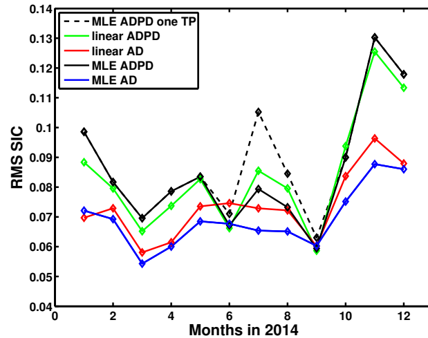
Figure 9. Comparison against OSI-SAF, of one tie-point (black dotted line) vs two tie-points (black plane line) with MLE; and MLE vs linear retrieval techniques. If not defined in the labels it is two tie-points.
