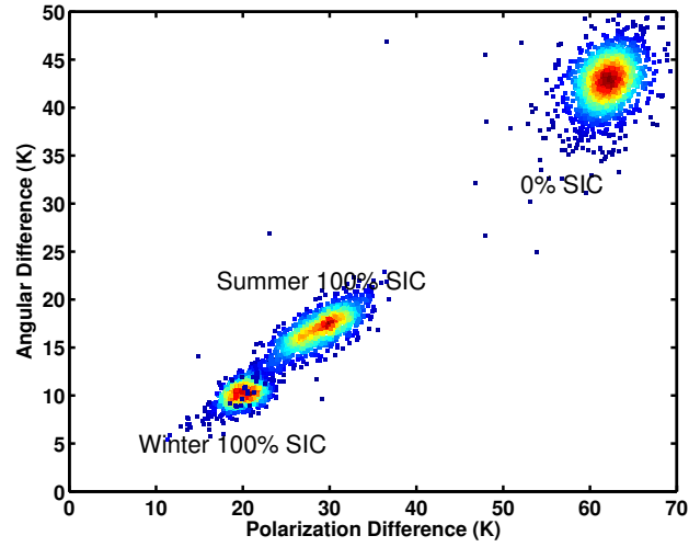
Figure 8. Scatter plot of the angular difference vs polarization difference in March and July 2014, with (red-to-blue) high-to-low index occurrence values for the two regions for generating tie-points, i.e., 0% and 100% sea ice concentration (SIC).
