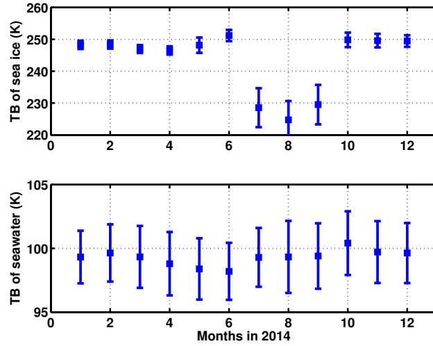
Figure 6. Temporal variation of the average brightness temperature T_B at nadir for (top) multi-year sea ice and (bottom) seawater at the two regions for generating tie-points. Note the factor of 4 change in the vertical scales.
