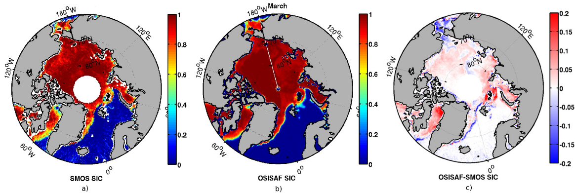
Figure 11. SMOS SIC with MLE (a), OSISAF SIC (b) and the differences (c) for 3rd March 2014.
