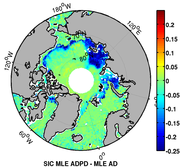
Figure 10. SMOS SIC with MLE AD+PD minus SMOS SIC with MLE AD inversion techniques.
