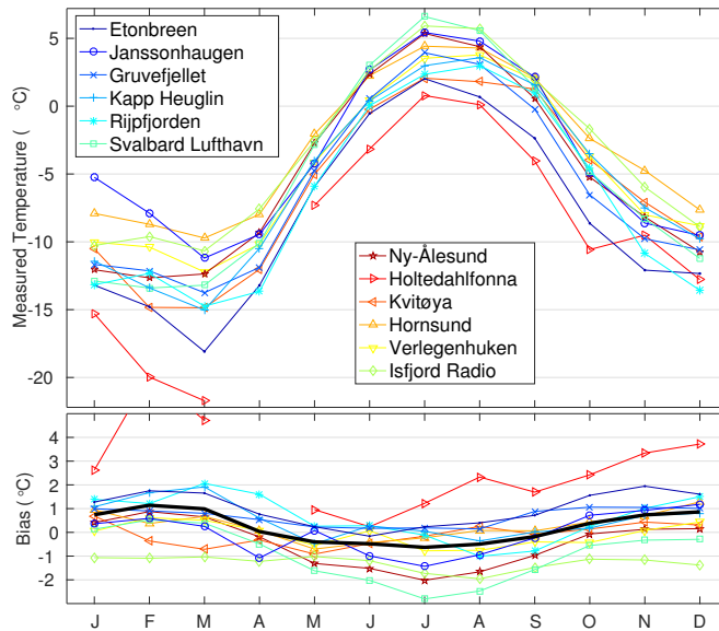
Figure 5. Observed monthly mean 2 m air temperatures (upper panel) and biases given by downscaled minus observational monthly averages (lower panel). Bold black line is average over the 12 sites.
