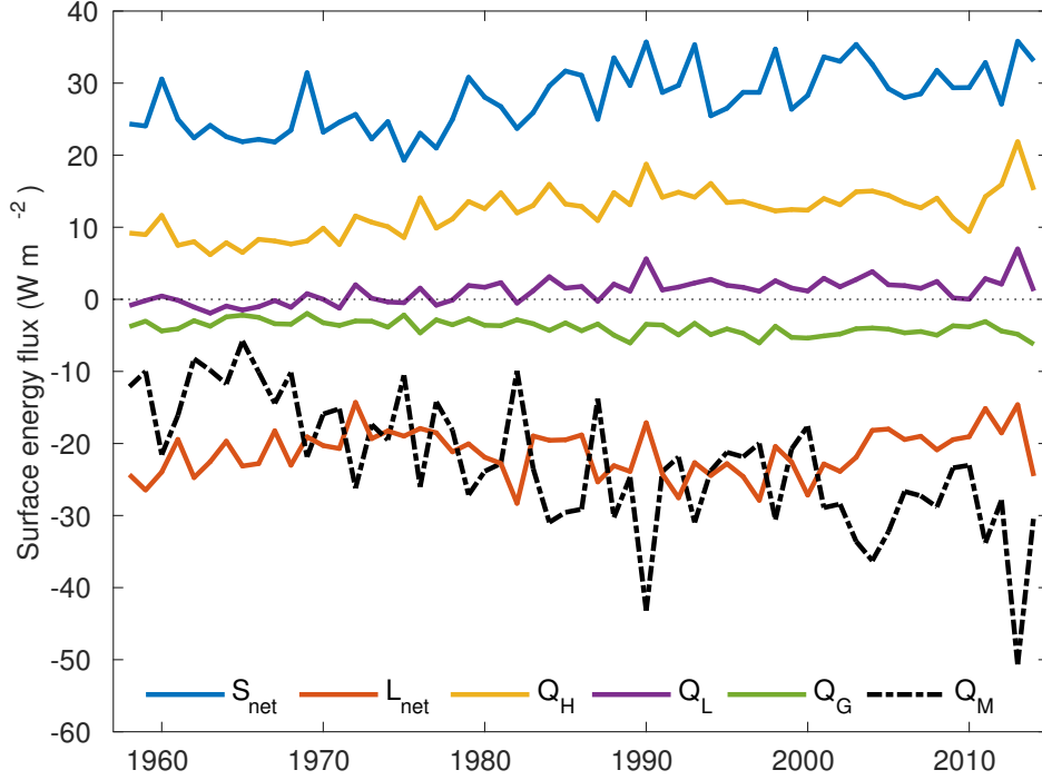
Figure 8. Modeled energy fluxes ( \text{W m}^{-2} ) averaged over all glaciers and each year's melt season (15 May- 30 Sept.) for the period 1957-2014. Area averaging was performed based on each year's glacier mask.
