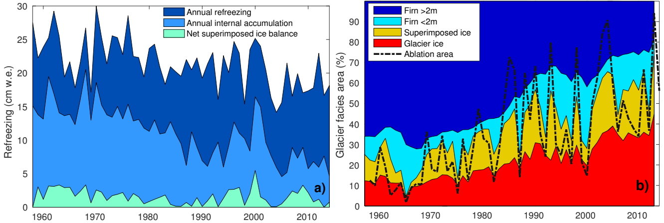
Figure 10. a) Annual refreezing, and internal accumulation (i.e. refreezing below the previous summer surface) and the net superimposed ice balance, i.e. the amount of superimposed ice at the end of each mass-balance year. b) Annual fractional areal extent of glacier facies divided into glacier ice, superimposed ice, thin firm (<2 m) and thick firm (>2 m).
