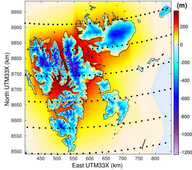
Figure 3. Elevation difference (m) between the ERA topography and the 1-km DEM; negative values mean that ERA elevations are lower. Black dots show the 0.75^\circ \times 0.75^\circ ERA grid.
