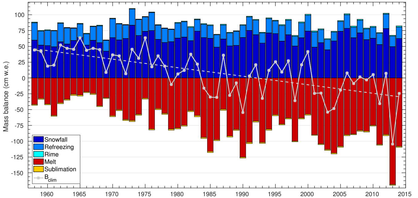
Figure 7. Annual specific climatic mass balance ( B_{\text{clim}} ) and its components, 1957-2014. Area averaging is performed using the temporal glacier mask. Dashed line is the linear mass balance trend of -14 \pm 4.1 cm w.e. decade ^{-1} , with uncertainty referring to two standard deviations.
