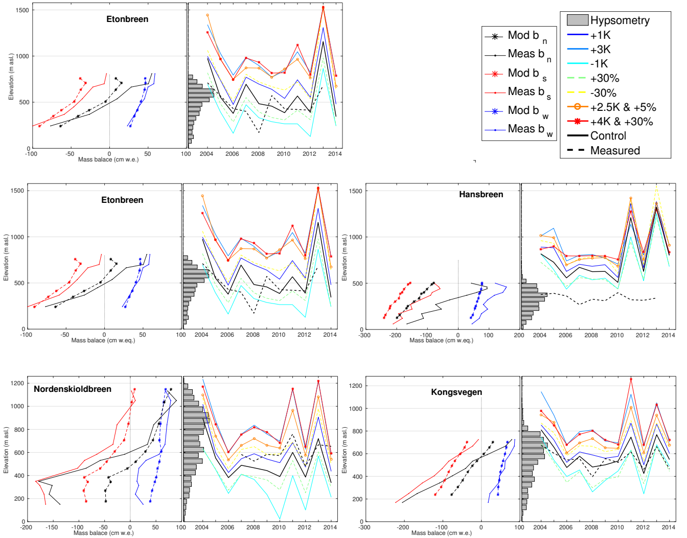
Figure 11. Modeled and measured seasonal mass balance gradients (left panels of each glacier's subplot) at the five validation glaciers averaged over the period 2004-2013 (right panels). Modeled results include the control run and sensitivity experiments. Dots and stars mark the altitudes of the measurement sites and corresponding DEM grid cell, respectively. Grey bars show area-altitude distribution for 50 m elevation bins. Note that the mass balance measurements at Kongsvegen, Etonbreen and Hansbreen over 2004-2013 also are used for model calibration,
