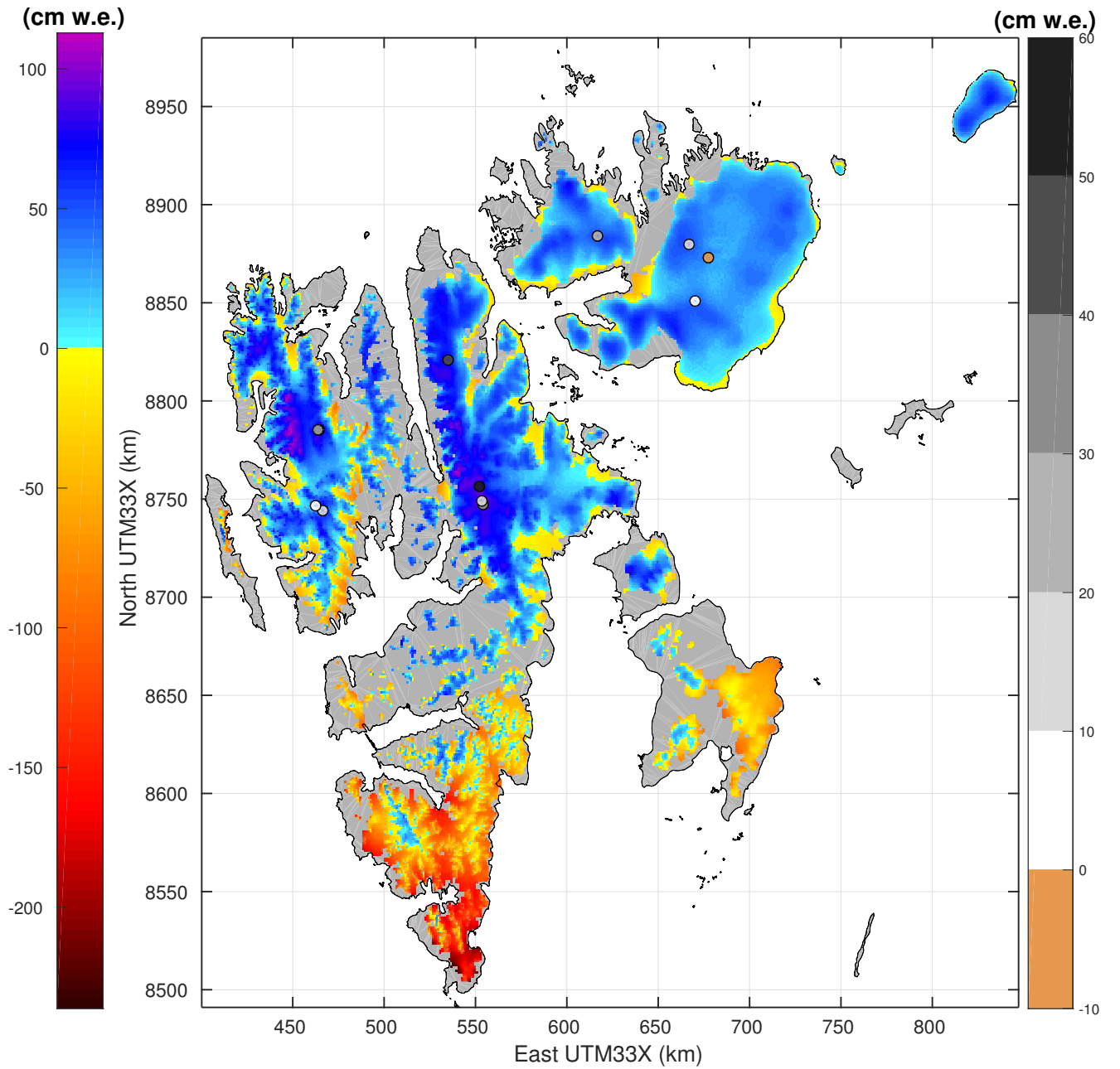
Figure 6. Map of simulated specific climatic mass balance ( B_{\text{clim}} ) averaged for the period 1957-2014 in \text{cm w.e. yr}^{-1} (colorscale on left side). Circles indicate difference between modeled B_{\text{clim}} and the ice core derived B_{\text{clim}} (colorscale on right side). For several ice cores mass balance estimates are available for different time periods, here we only show the longest period; see Table 7 for details.
