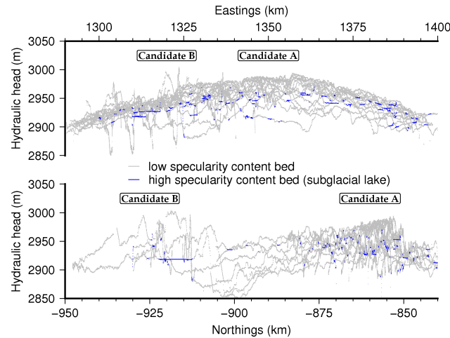
Figure 4. The OIA extracted bed data projected into hydraulic head (the water level equivalent to the pressure imposed by the ice overburden), and viewed in the projected Northing plane (lower, looking across the ice divide) and projected Easting plane (upper, looking along the ice divide). Regions of high specularity content (subglacial lakes) are highlighted in blue. Note that lakes are flat, indicating hydrostatic equilibrium. Many of the subglacial lakes lie in valleys that cut into the primary surface that envelopes the local subglacial topography; only one is found above the 2950 m head level. Projection for the horizontal axis Eastings and Northings is Antarctic Polar Stereographic.
