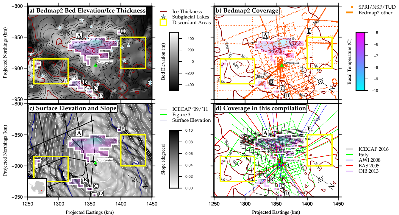
Figure 2. Dome C in the context of the Van Lieffering and Pattyn (2013) frozen bed candidates and Concordia Station. A threshold of -5^{\circ}\text{C} was used for selecting candidates. Bedmap2 bed elevation and ice thickness contours (Fretwell et al., 2013) are shown in panel a, along with subglacial lakes known as of Wright and Siegert (2012). Regions where trends seen in surface data are absent in Bedmap2 are shown by the yellow boxes in all panels. Coverage used to constrain Bedmap2 (orange) is shown in panel b, with the 1970s SPRI/NSF/TUD dataset being the sparse, dotted lines. Surface elevation and slope from Cryosat-2 (Helm et al., 2014) is shown in panel c, with older ICECAP tracks (Cavitt et al., 2016) in black and a green line showing the ice divide profile shown in Fig. 3. ICECAP Old Ice A data discussed in this paper (black), as well additional modern datasets are shown in panel d. Contours in c and d are Bedmap2 ice thickness. Projection is Antarctic Polar Stereographic, and the region corresponds to the red box in Fig. 1
