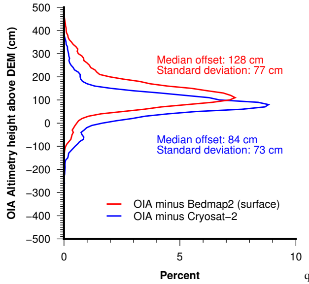
Figure 7. Histograms comparing 2 surface elevation DEMs (largely derived from radar altimetry) and OIA altimetry. Expected accuracy of OIA altimetry is 15 cm (Young et al., 2015).
