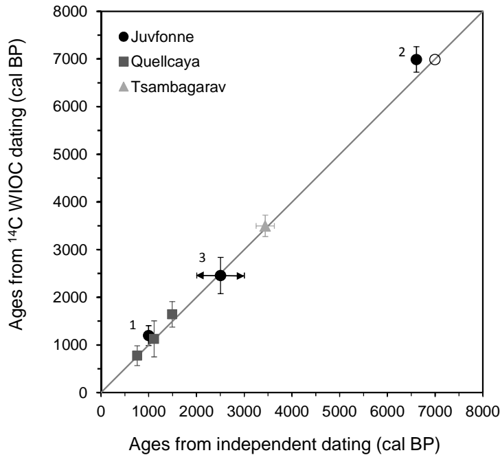
Figure 3: Scatter plot showing the ages obtained with the WIOC ^{14}\text{C} method for independently dated ice, including the conventionally ^{14}\text{C} dated Juvfonne organic-rich layers (Ødegård et al., 2016), the ^{14}\text{C} dated fly found in the Tsambagarav ice core, and the Quelccaya ice dated by annual layer counting (Thompson et al., 2013). Error bars denote the 1\sigma uncertainty. Note that the Juvfonne WIOC samples and the organic-rich layers were not sampled from the exact same depth, but adjacent to each other. For the youngest (1) and oldest (2, containing the plant fragment) the ice for WIOC ^{14}\text{C} analysis was sampled below the layers whereas the third sample (3) was bracketed by two layers. For (3) the arrow thus indicates the age range between the lower and upper 2\sigma boundary of these two layers, respectively. For (2) the open circle indicates an estimated age for the according WIOC ice sampling depth based on a fit through all the conventionally dated organic-rich layers, presented in Ødegård et al., 2016).
