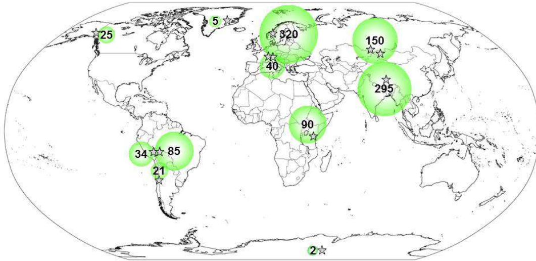
Figure 2: World map showing the sites from which ice samples were analysed with the ^{14}\text{C} method (gray stars): Edziza, Canada, 57.71^\circ\text{ N } 130.63^\circ\text{ W} ; GRIP, Greenland, 72.59^\circ\text{ N}, 37.65^\circ\text{ W} , 3230 m a.s.l.; Juvfonne, Norway, 61.68^\circ\text{ N}, 8.35^\circ\text{ E} ; Colle Gnifetti, Switzerland, 45.93^\circ\text{ N}, 7.87^\circ\text{ E} ; Mt. Ortles, Italy, 46.51^\circ\text{ N}, 10.54^\circ\text{ E} ; Belukha, Russia, 49.80^\circ\text{ N}, 86.55^\circ\text{ E} ; Tsambagarav, Mongolia, 48.66^\circ\text{ N}, 90.86^\circ\text{ E} ; Naimonanjia, China 30.45^\circ\text{ N}, 81.54^\circ\text{ E} ; Kilimanjaro, Tanzania, 3.06^\circ\text{ S } 37.34^\circ\text{ E} ; Quelccaya, Peru, 13.93^\circ\text{ S}, 70.83^\circ\text{ W} ; Nevado Illimani, Bolivia, 16.03^\circ\text{ S}, 67.28^\circ\text{ W} ; Mercedario, Argentina, 31.97^\circ\text{ S}, 70.12^\circ\text{ W} ; Scharffenbergbotnen, Antarctica, 74.00^\circ\text{ S}, 11.00^\circ\text{ W} . The average WIOC concentration in \mu\text{g}/\text{kg} at each site is indicated with green bubbles.
