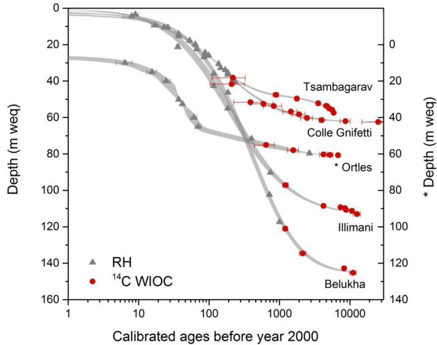
Figure 6: Compilation of age-depth relationships for five different ice cores, highlighting the importance of the WIOC 14 C dating to obtain continuous chronologies and to constrain the very specific glaciological conditions and settings of each site. For simplicity only reference horizons and 14 C dates were included. Gray triangles indicate reference horizons (RH) and red circles the 14 C-WIOC ages both plotted with 1σ uncertainties (smaller than the symbol size in some cases). For the Mt. Ortles core 210 Pb dated horizons with a larger uncertainty were used as RH due to the lack of absolute time markers prior to 1958; the gray triangle at 57.8 m weq depth is the conventional 14 C age of the larch leaf. Gray shaded areas represent the 1σ range of the respective fit for retrieving a continuous age depth relationship. For sample details and the fitting approaches applied, see main text and Table 1. References to the original data are summarized in Table 1. Note that for better visibility (avoiding overlap with Tsambagarav and Colle Gnifetti) the curve for the Mt. Ortles glacier was shifted down by 20 m and refers to the right-hand y-axis (*). 655 660
