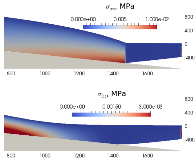
Figure 2. Stress tensor component \sigma_{xz} ( internal shear stress ) shown at the end of the ADVA experiment for SR1 (top) and SR3 (bottom) for the seaward 1000 km of the domain. At the base of the ice this approximates the basal shear stress, given the low slope of the bed. Note the different colour scales. Distance from the ice divide is shown along the bottom in km. Height relative to sea level is shown at the right end of the plots in m. Bedrock is shaded in grey. Vertical exaggeration is 200 times.
