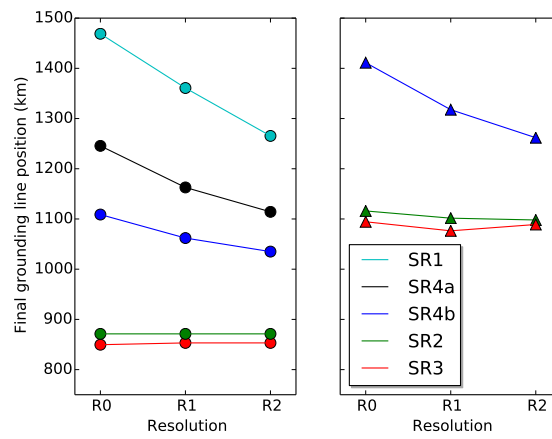
Figure 4. Final grounding line position (after 40 ka) against resolution (Table 2) for the retreat due to butressing reduction (RB, left panel) and retreat due to basal melting (RHW, right panel) with the different sliding relations (Table 1). The y-axis range is identical in both panels. The vertical ordering of the families of curves matches that of the legend tables.
