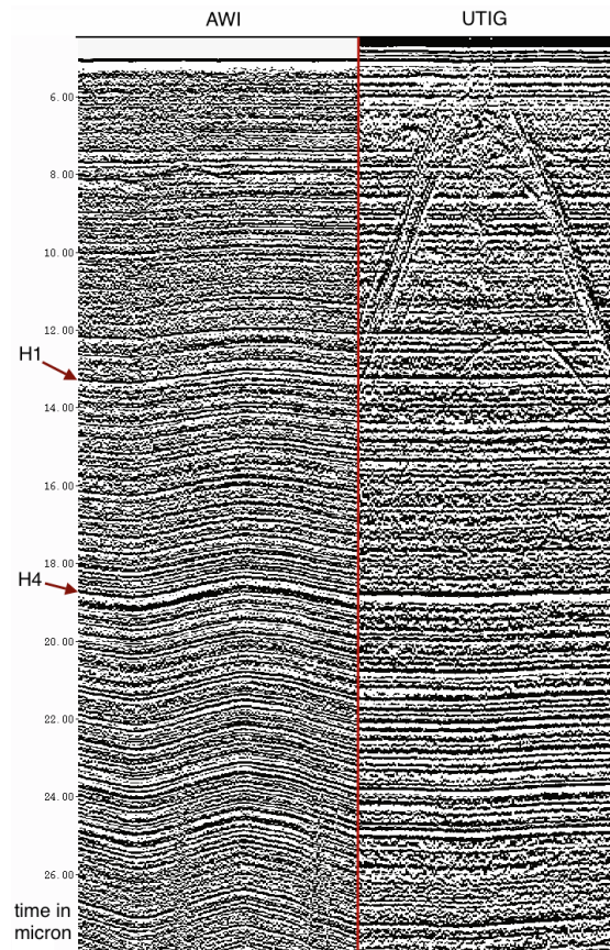
Figure 4. Intersection of AWI and UTIG profiles for direct visual comparison. Two examples of identified IRHs are indicated by red arrows. Note that the air-ice reflection is shifted to 5 \mu\text{s} . All strong horizons can be traced smoothly across the intersection.
