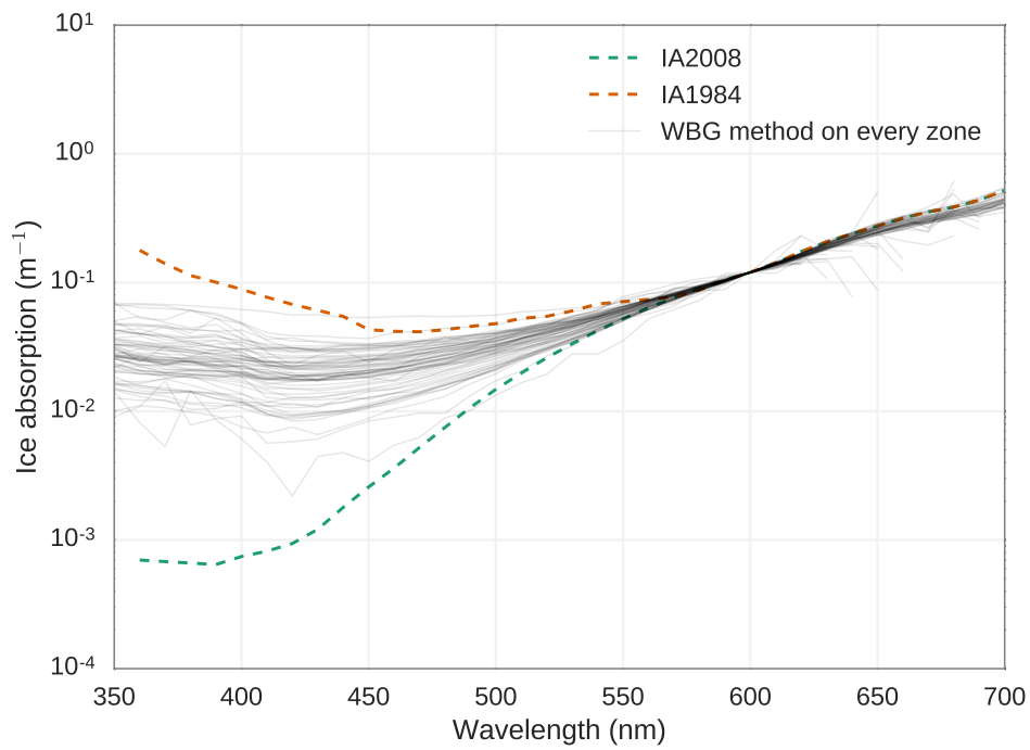
Figure 5. Ice absorption spectra estimated by the WBG Method (Warren et al., 2006) on the 70 homogeneous zones selected in zone from the selection on the 56 radiance profile profiles measured around Concordia.
