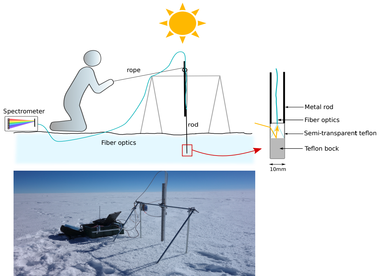
Figure 1. Scheme and picture of SOLEXS. The rod (black) is vertically guided and inserted in the snow with the rope manipulated by the operator. The quadrupod (gray) is oriented to minimize the shadows. At the bottom end of the rod, the light first traverses the semi-transparent 0.5-mm thin teflon cylinder and is reflected by a teflon block towards the fiber tip from where it is transferred transferred to the spectrometer.
