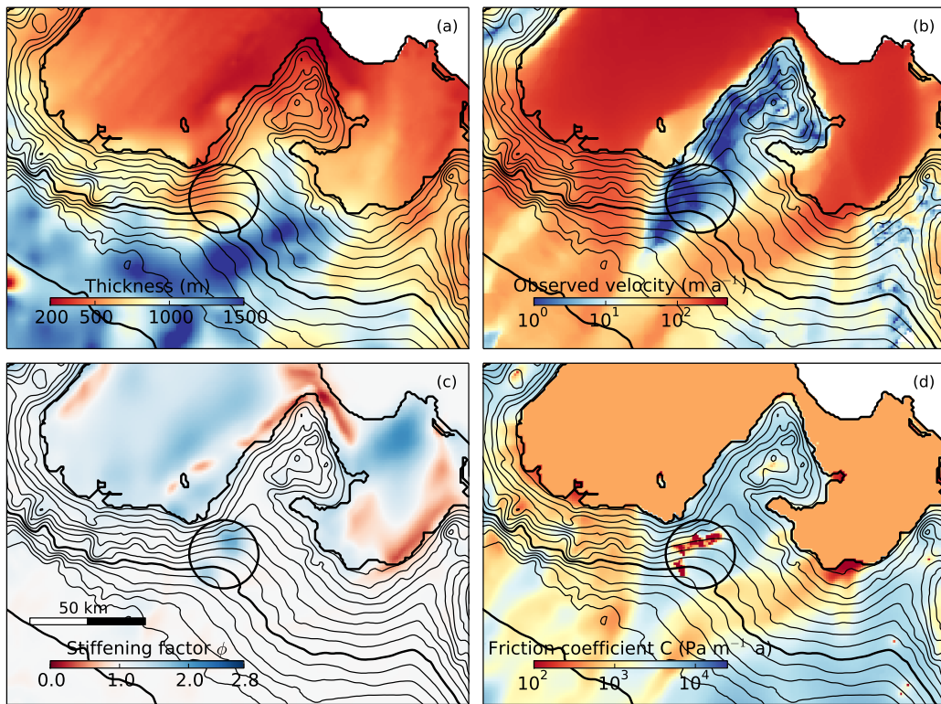
Supplementary Figure 1. Results of the data assimilation for linear sliding showing a zoom in over an area with velocity mismatch (shown by a circle). (a) Thickness, (b) observed velocities, (c) stiffening factor and (d) friction coefficient. Contours show ice surface height every 50 m in the range 100-800 m.
