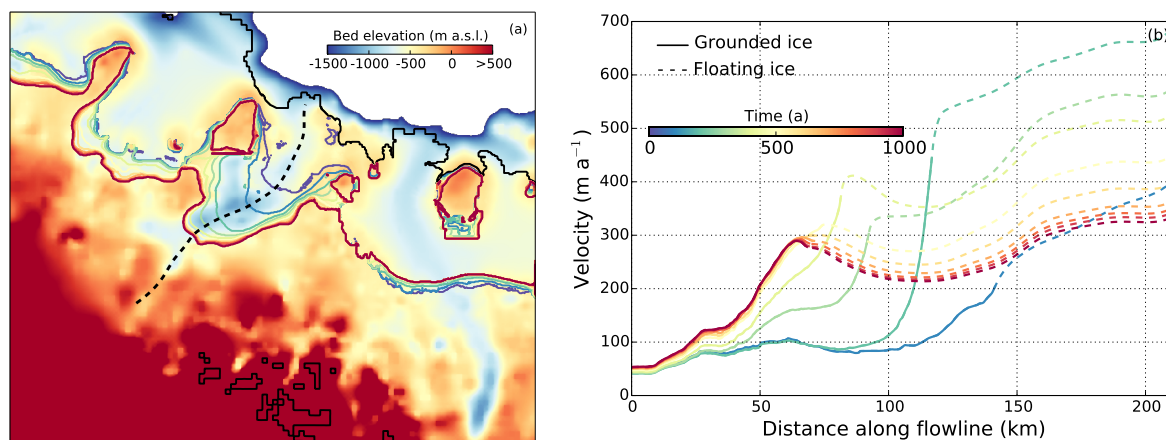
Figure 6. Grounding-line migration for the B_e/S/L/M_{b1}/A_m experiment. (a) Bed elevation in the background, grounding lines are shown every 100 years (colorscale shown in (b)) and the dashed line shows the central flowline of HB. (b) Ice velocity profiles along the central flowline of HB, shown every 100 years. The grounding-line position is marked by the limit between solid and dashed parts of profiles.
