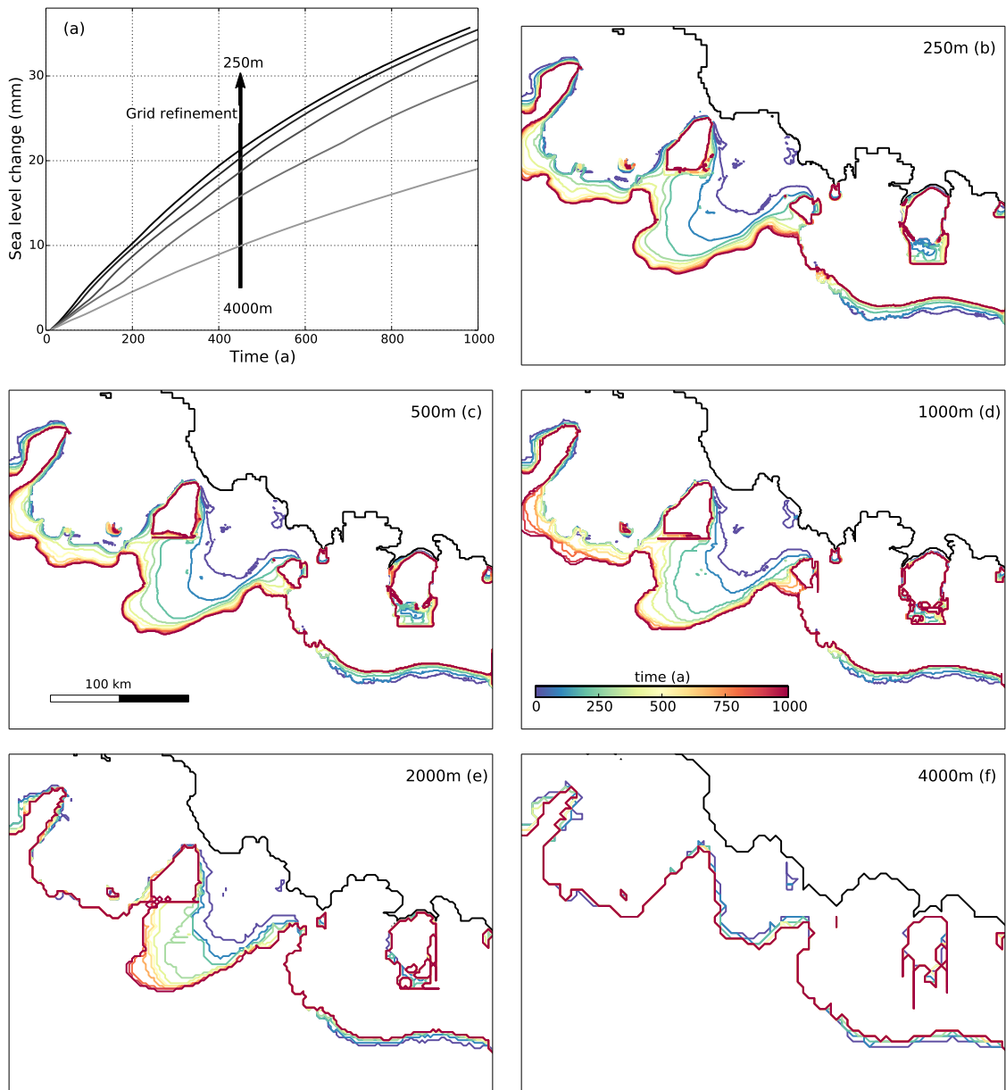
Supplementary Figure 2. sensitivity to grid resolution between 250 m and 4000 m at the grounding line, performed for the B_e/S/L/M_{b1}/A_m experiment. (a) Cumulative sea level changes. The 4000 m resolution give the lowest changes while the 250 m resolution gives the highest changes. The differences between 250 m and 500 m are not significant. The 500 m resolution has therefore been chosen to run all the simulations discussed in the main paper. (b) to (f) Grounding-lines shown every 100 years (colorscale shown in (d)) for the resolution indicated at the top right of each panel.
