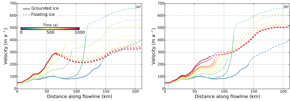
Supplementary Figure 3. Ice velocity profiles shown every 100 years for the (a) B_e/S/L/M_{b1}/A_m experiment along the flowline shown in Figure 6(a), and (b) for the same experiment in which the sub ice-shelf melting is switched off beneath the Hansenbreen ice shelf when its retreating grounding enters the upsloping part of the bed. The sub ice-shelf melting for other parts of the computational domain are not altered. The grounding line position is marked by the limit between solid and dashed parts of profiles.
