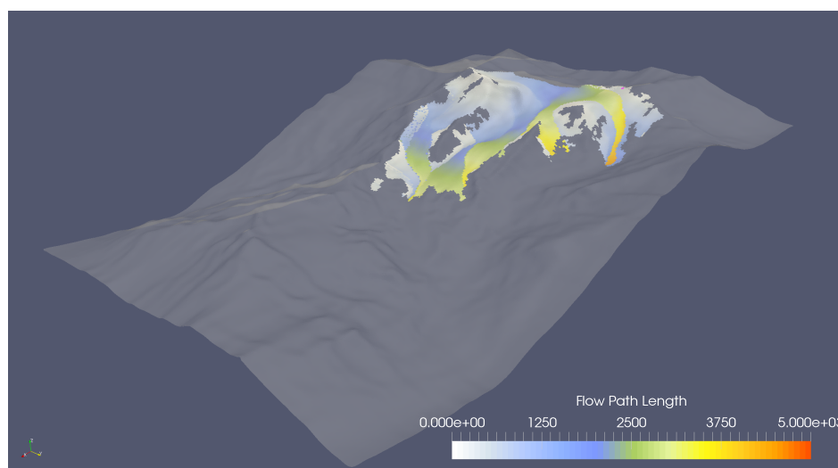
Fig. 1. Calculated flow path lengths
