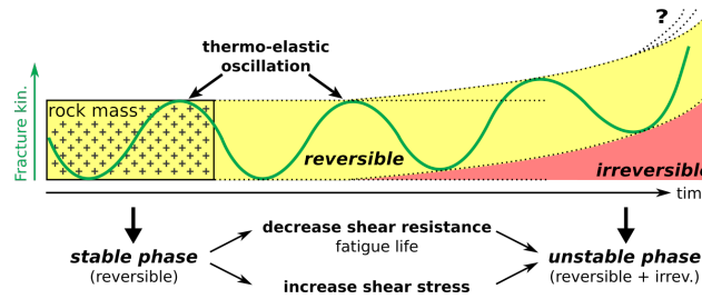
Figure 2. Evolution of a permafrost affected rock mass with persistent thermo-elastic oscillations: initially reversible displacement of rock mass can develop an additional irreversible component either by an increase in shear stress or by a decrease in shear resistance.
