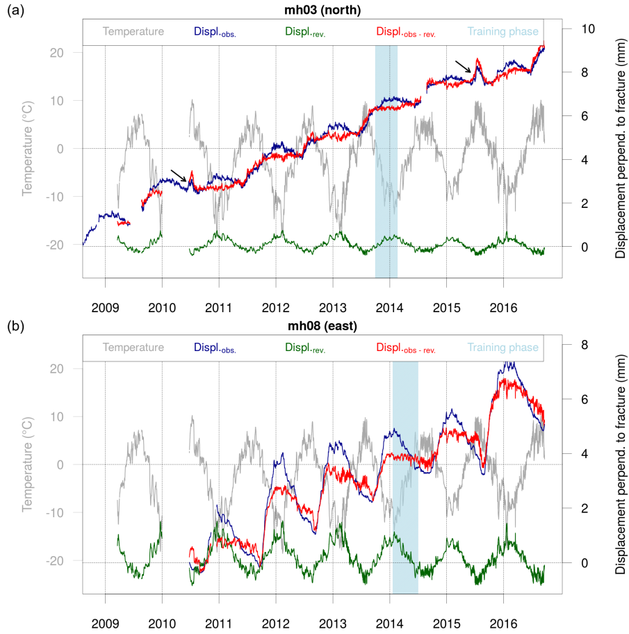
Figure 8. LRM (green) applied to the observed displacements (blue) perpendicular to the fracture at location mh03 (a) and mh08 (b). The reversible component (green) due to thermo-elastic strains in rock can be modeled by a linear regression model (LRM) with temperature (dark gray) and displacement measurements during a training period of several months (light blue shading) as input data. Subtracting these reversible displacements from the observed data results in the red line, referred to as irreversible fracture displacement.
