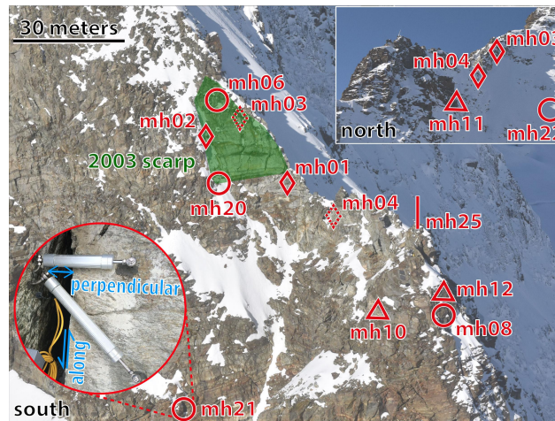
Figure 5. Overview of crackmeter installations. Location mh01–mh04 (indicated with \diamond ) are instrumented with one crackmeter perpendicular to the fracture. Location mh06 , mh08 and mh20–mh22 (indicated with \circ ) are instrumented with two crackmeters to calculate displacements perpendicular to and along fracture. Temperature measurements in fractures exist at most location. Locations with only rock temperature measurements are indicated with \triangle while for the weather station | is used. Scarp of the 2003 rockfall is shaded green.
