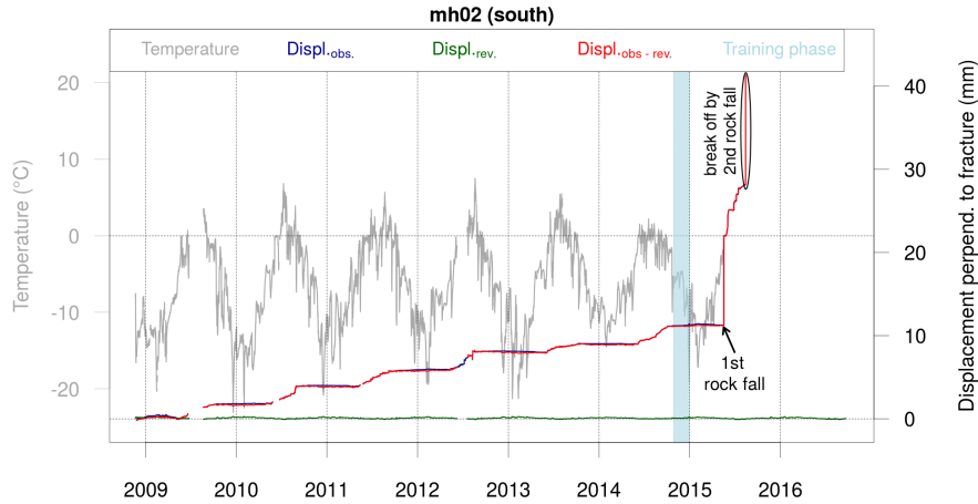
Figure 12. LRM (green) applied to the observed displacements (blue) perpendicular to the fracture at location mh02 . The reversible component (green) due to thermo-elastic strains in rock can be modeled by a linear regression model (LRM) with temperature as input data (dark gray) and displacement measurements during a training period of several months (light blue shading). Subtracting these reversible displacements from the observed data results in the red line, referred to as irreversible fracture displacement.
