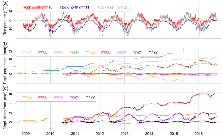
Figure 6. Thermal conditions and fracture displacements at the Matterhorn Hörnligrat field site over a course of eight years: (a) The thermal conditions are shown by characteristic rock temperatures for the south, east and north side of the ridge measured at a depth of 0.85 m. The fracture kinematics are shown as normalized displacements (b) perpendicular to and (c) along fractures. A gap in the rock temperature time series of location mh12 ( T_{\text{east}} ) is filled for the time period November 2012 until July 2013 and from August 2014 onwards applying quantile mapping using the best regressors approach (Staub et al., 2016) with a coefficient of determination R^2 = 0.92 .
