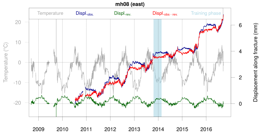
Figure 13. LRM (green) applied to the observed displacements (blue) along the fracture at location mh08 . The reversible component (green) due to thermo-elastic strains in rock can be modeled by a linear regression model (LRM) with temperature as input data (dark gray) and displacement measurements during a training period of several months (light blue shading). Subtracting these reversible displacements from the observed data results in the red line, referred to as irreversible fracture displacement.
