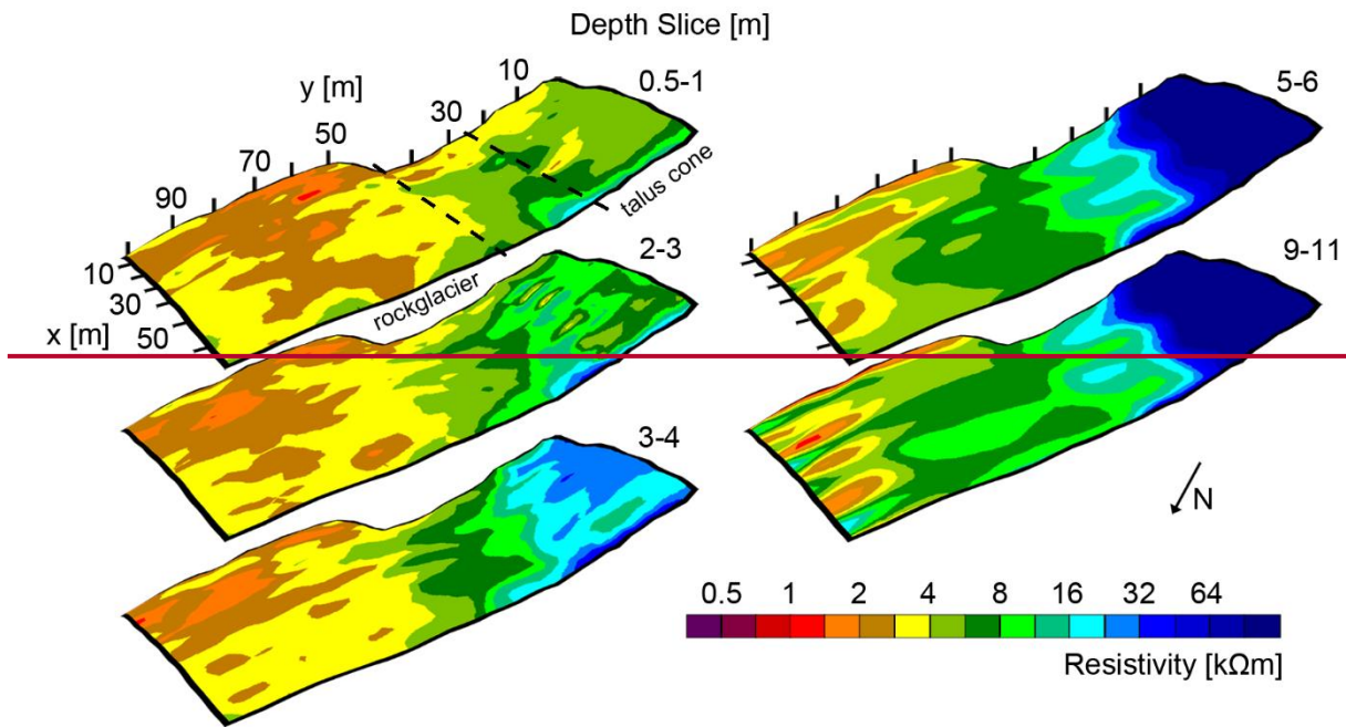
Fig. 54: Selected depth slices of the quasi-3D ERI model Nair. Quasi-3D ERI Model Nair. Chosen depth slices.
