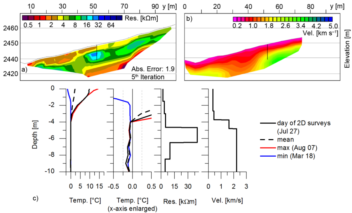
Fig. 43: Comparative analysis of (a) 2D ERT Profile, (b) 2D SRT Profile and (c) 1D Temperature/ Resistivity/ P-wave v-Velocity plots profiles at Uertsch rockglacier. Profiles of resistivity and P-wave velocity are extracted from the tomograms above at the borehole position.
