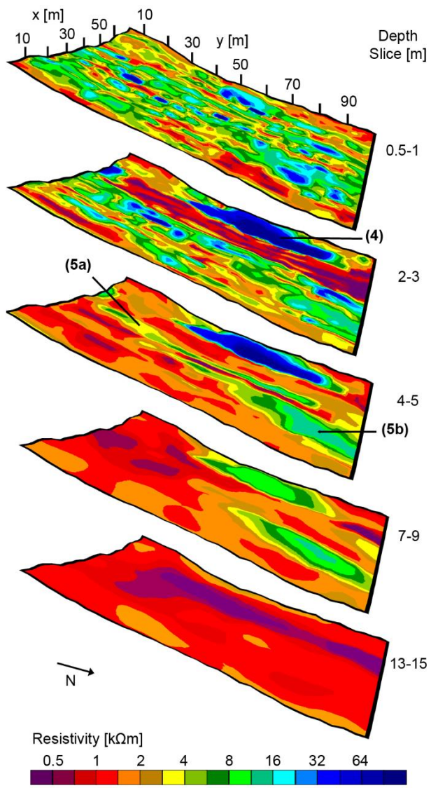
Fig. 76: Selected depth slices of the quasi-3D ERI model Uertsch_02. Numbers refer to structures described in the text. Quasi-3D ERI Model Uertsch_02. Numbers refer to structures described in the text. Chosen depth slices.
