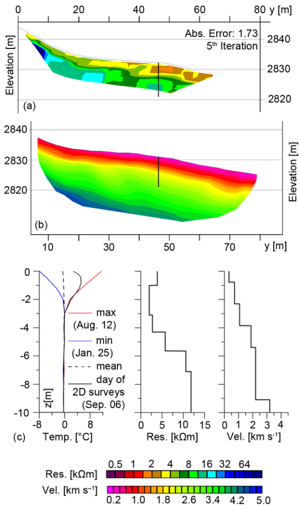
Fig. 3: Comparative analysis of (a) 2D ERT Profile, (b) 2D SRT Profile and (c) 1D Temperature/ Resistivity/ Velocity plots of Nair rockglacier.
