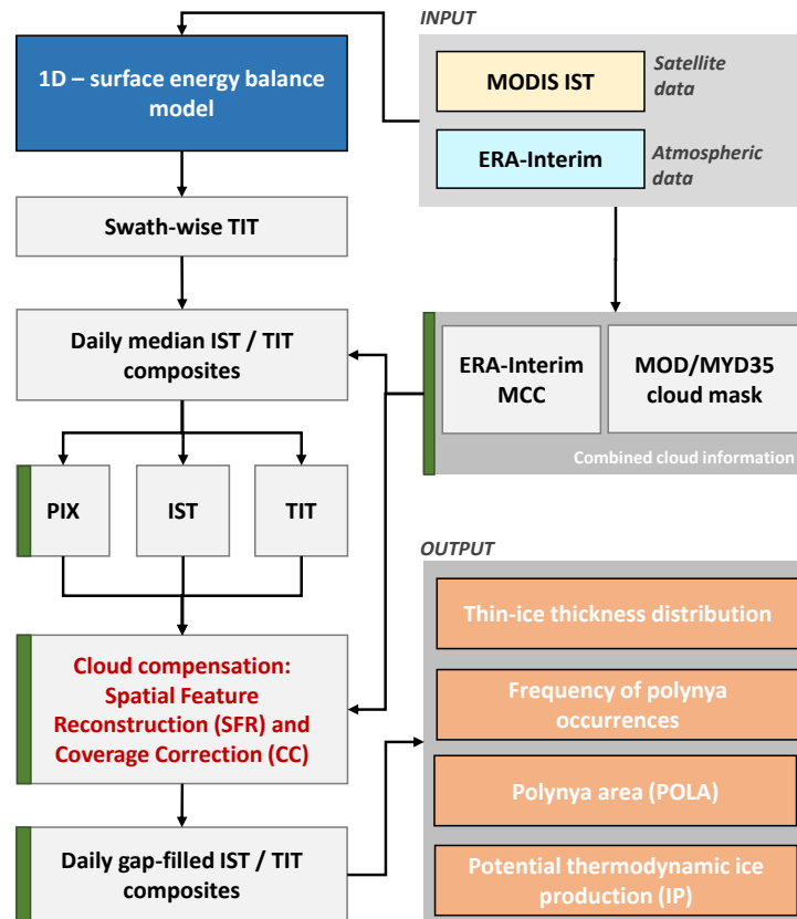
Figure 2. Schematic overview on the current version of the MODIS thin-ice thickness (TIT) retrieval scheme, based on Paul et al. (2015b) and Preußner et al. (2015a). The most recent updates are marked in green and are mainly aimed towards an additional cloud-cover treatment. Besides indicated abbreviations, 'IST', 'MCC' and 'PIX' denote the ice surface temperature, medium cloud cover and persistence index, respectively.
