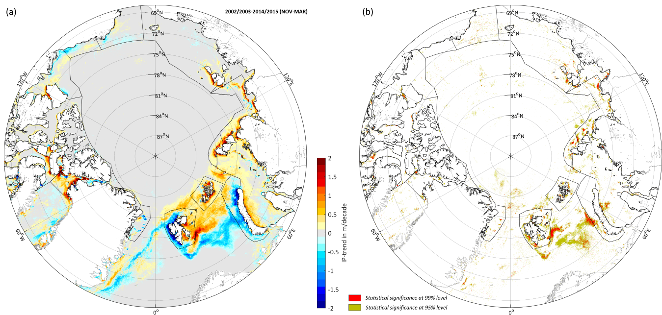
Figure 8. (a) Decadal trends (m per decade) of wintertime (November to March) ice production in the Arctic, north of 68^{\circ} N. Trends are calculated by applying a linear regression on the annual accumulated IP per pixel for the period 2002/2003 to 2014/2015. Areas with statistical significance (based on a two-sided t-test) at the 95% and 99% level are depicted in (b). The margins of applied polynya masks (Fig. 1) are shown in black dashed lines.
