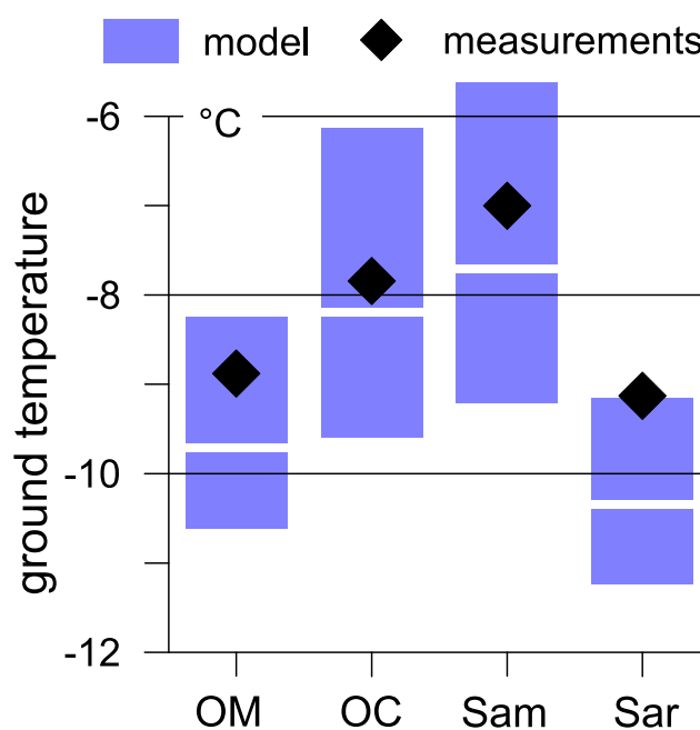
Figure 9. Modeled and measured annual average ground temperatures for the LRD boreholes for the two-year period September 2010 to August 2012 (OM: Olenyokskaya Channel mouth; OC: Olenyokskaya Channel center; Sam: Samoylov Island borehole; Sar: Sardakh Island). Blue bar: spread between model runs with snow densities of 200 and 250 kg m -3 ; white line: model run with snow density 225 kg m -3 . The ground temperatures correspond to the depths given in Figs. 7 and 8, for Samoylov, the simulations for the borehole stratigraphy (Sect. 4.2.1, Fig. 8 right) are presented.
