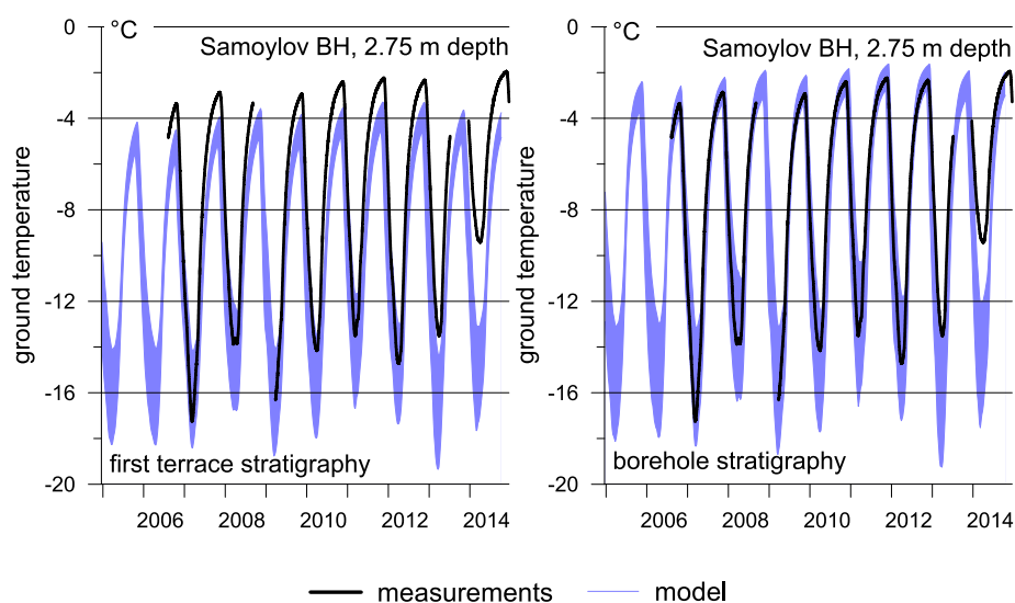
Figure 8. Modeled and measured ground temperatures for the borehole on Samoylov Island. Left: subsurface stratigraphy of the first terrace (Table 1). Right: stratigraphy adapted to the true ground conditions at the borehole (0-0.5 m: 30% water/ice, 10% air, 60% mineral, sand; 0.5-9 m: 40% water/ice, 60% mineral, sand; deeper layers as for first terrace, Sect. 4.2.1). The blue area depicts the spread between model runs with snow densities of 200 and 250 kg m -3 .
