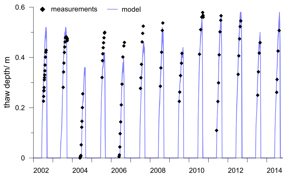
Figure 10. Modeled and measured thaw depths on Samoylov Island. The measurements correspond to the average of 150 locations on Samoylov Island (Boike et al., 2013). The average standard deviation of the measurements (i.e. the spatial variability of thaw depths) is 0.06 m. The blue area depicts the spread between model runs with snow densities of 200 and 250 kg m -3 .
