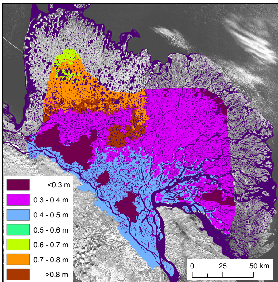
Figure 12. Modeled average maximum thaw depths for the period 2004-2013, with a snow density of 225 \text{ kg m}^{-3} .
