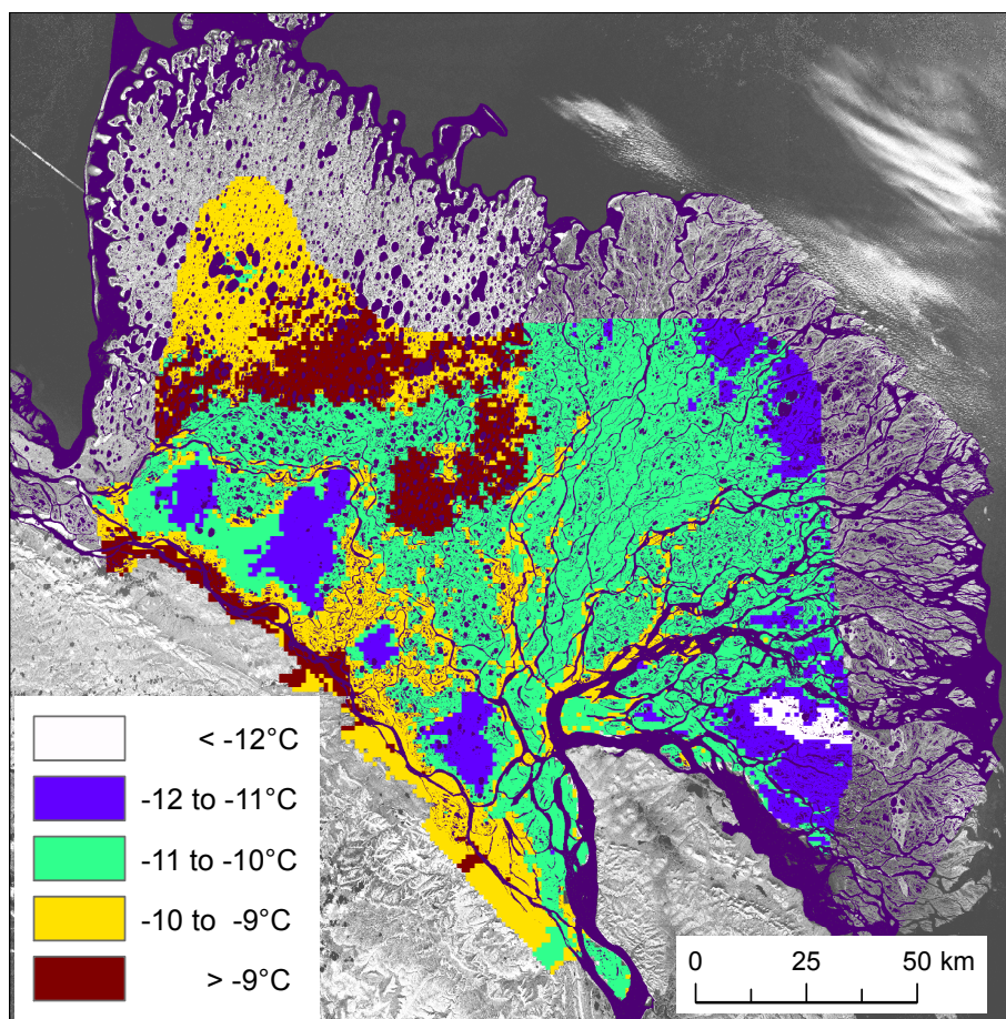
Figure 11. Modeled average ground temperatures at 1 m depth for the period 2004-2013, with a snow density of 225 kg m -3 .
